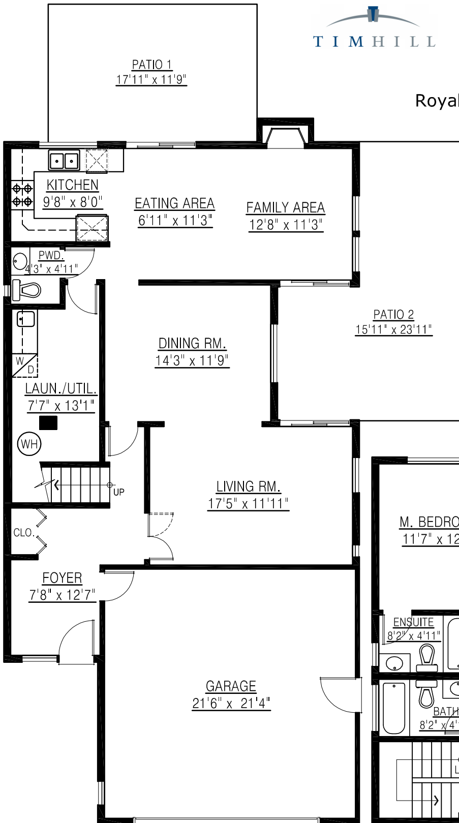
MAIN FLOOR PLAN FLOOR AREA: 1,114 sq.ft.
