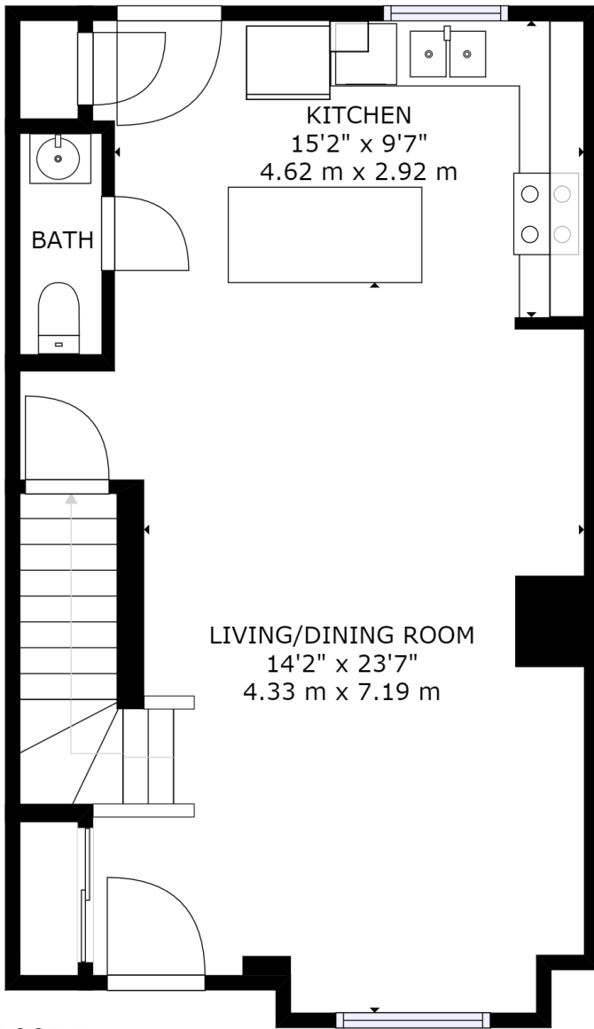
FLOOR 1
