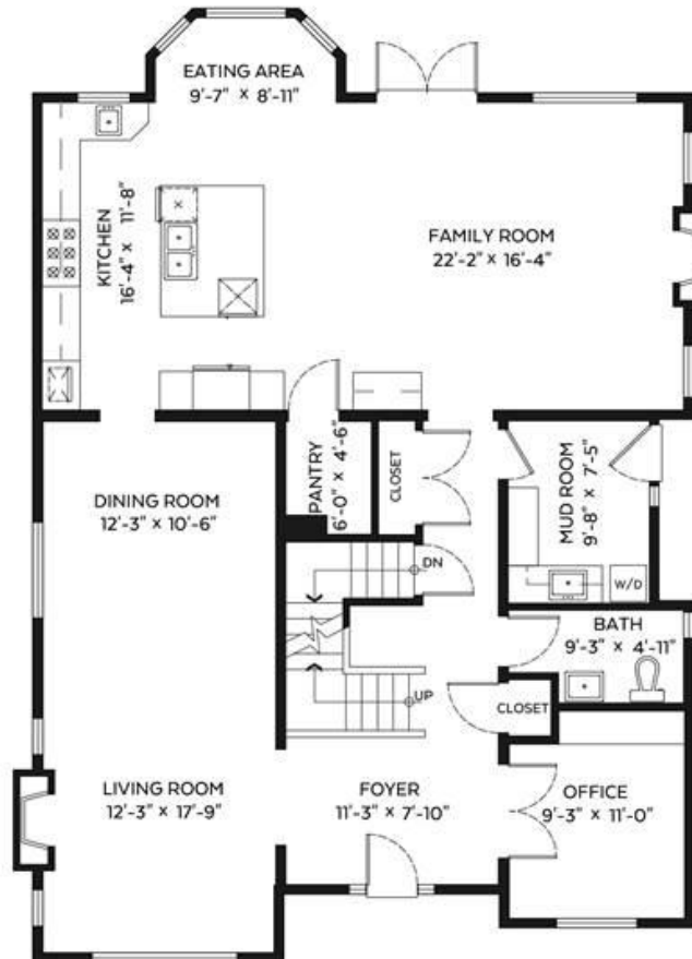
Main Floor Plan Floor Area: 1,574 sq.ft.
