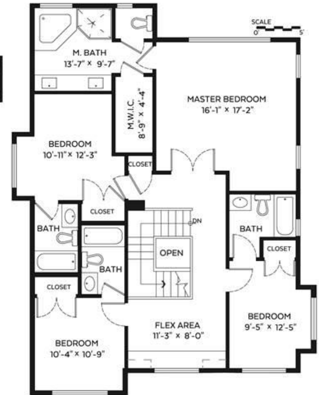
Upper Floor Plan Floor Area: 1,300 sq.ft.
