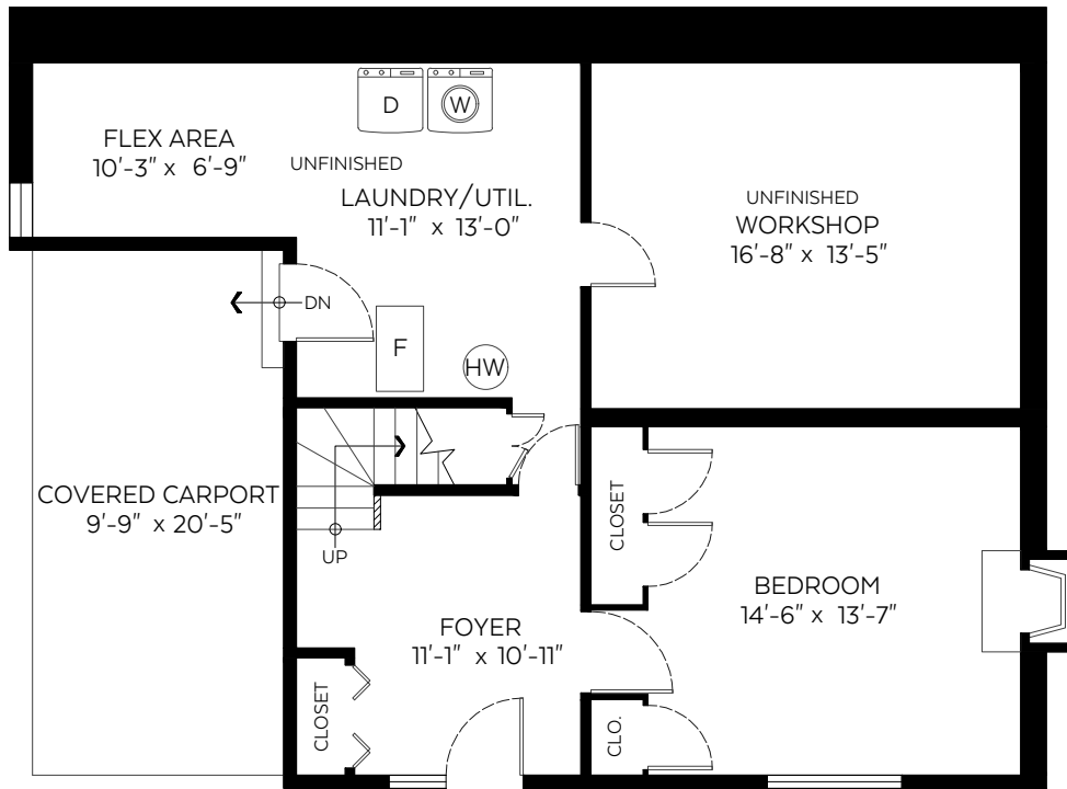
Lower Floor Plan Fin. Floor Area: 442 sq.ft. Unfin. Floor Area: 558 sq.ft. Ceiling Height: 9'-11"
