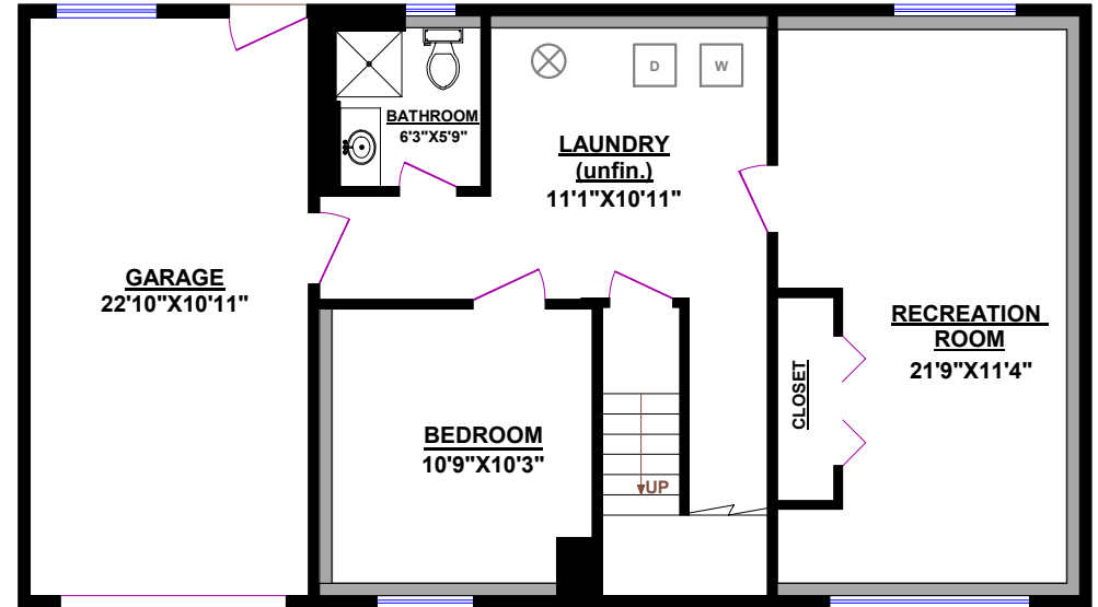
LOWER LEVEL
