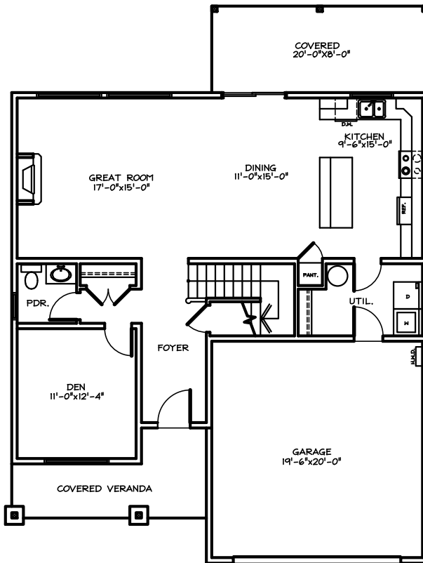
MAIN FLOOR PLAN 1074 SQ. FT. 2089 SQ. FT. TOTAL
