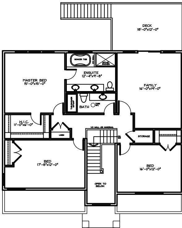
UPPER FLOOR PLAN 1470 SQ. FT.
