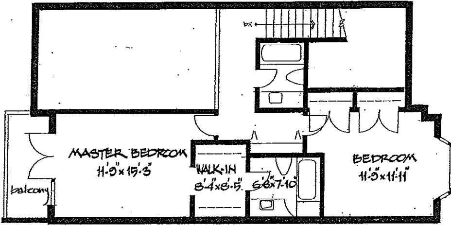
UPPER FLOOR
