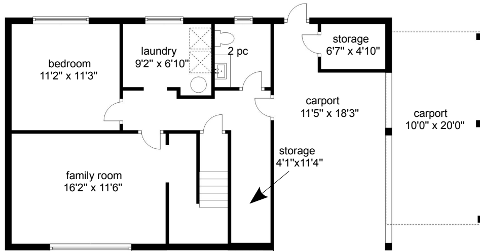
LOWER 672 sq ft General ceiling height 7'9"
