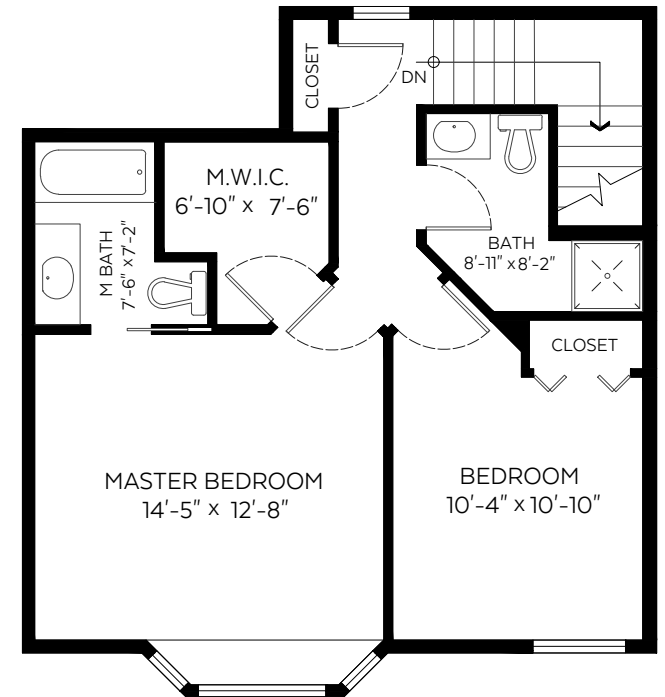
Upper Floor Plan Floor Area: 643 sq.ft
