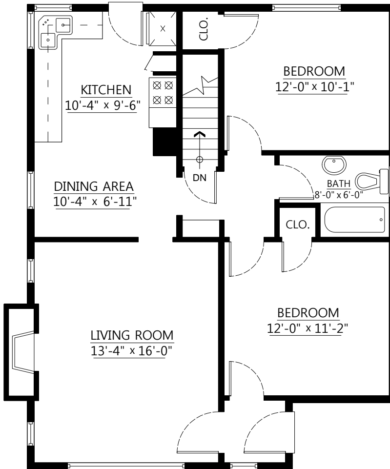
Main Floor Plan Floor Area: 865 sq.ft.
