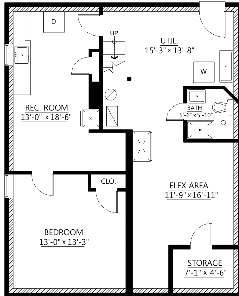
Lower Floor Plan Floor Area: 936 sq.ft.
