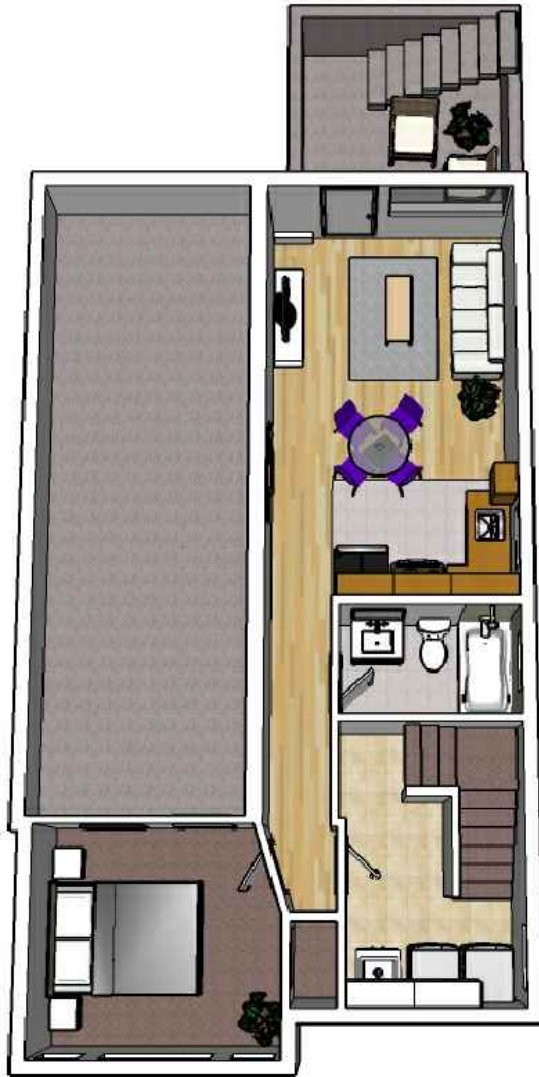
BASEMENT SUITE/ LOWER FLOOR PLAN
