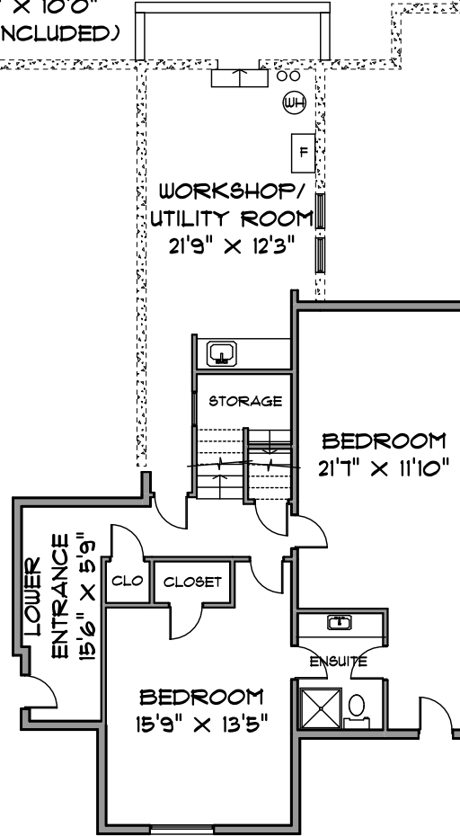
LOWER LEVEL 1317 SQ. FT.
