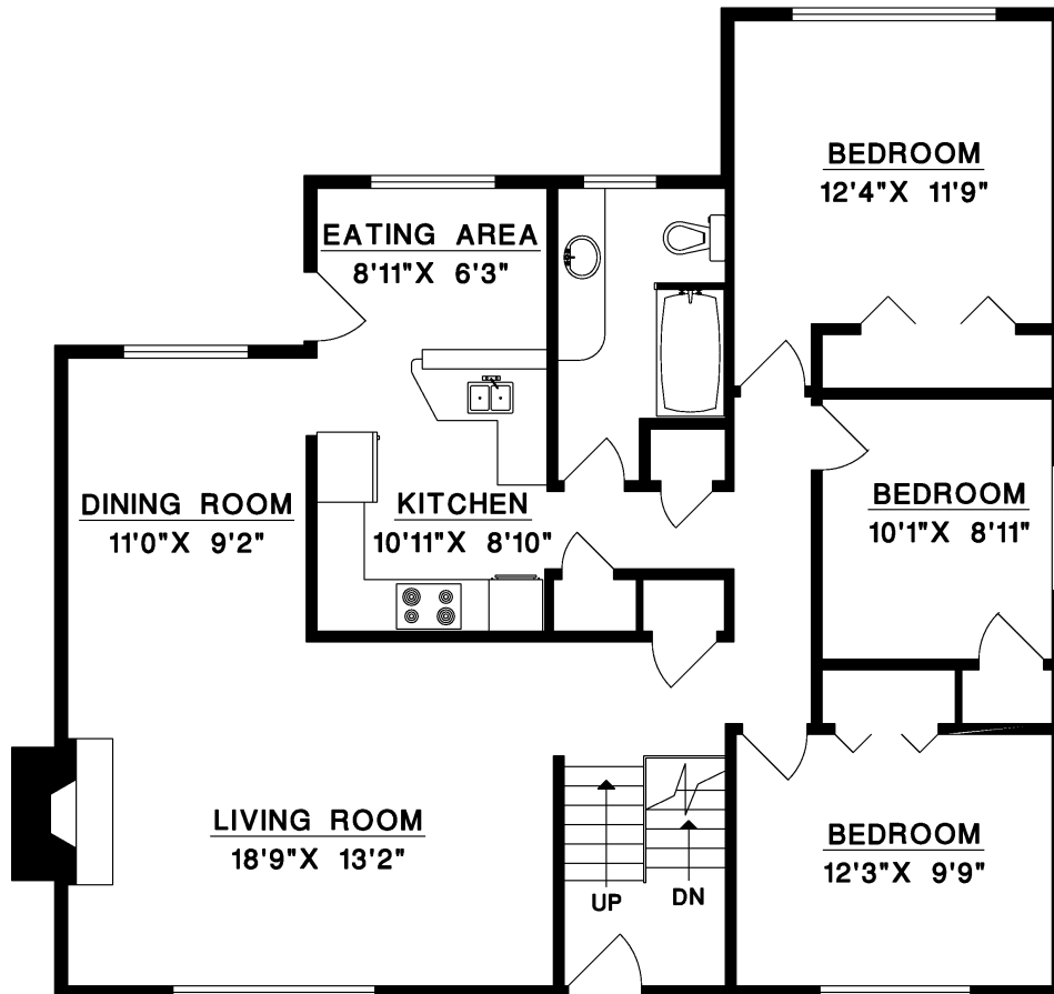
MAIN FLOOR
