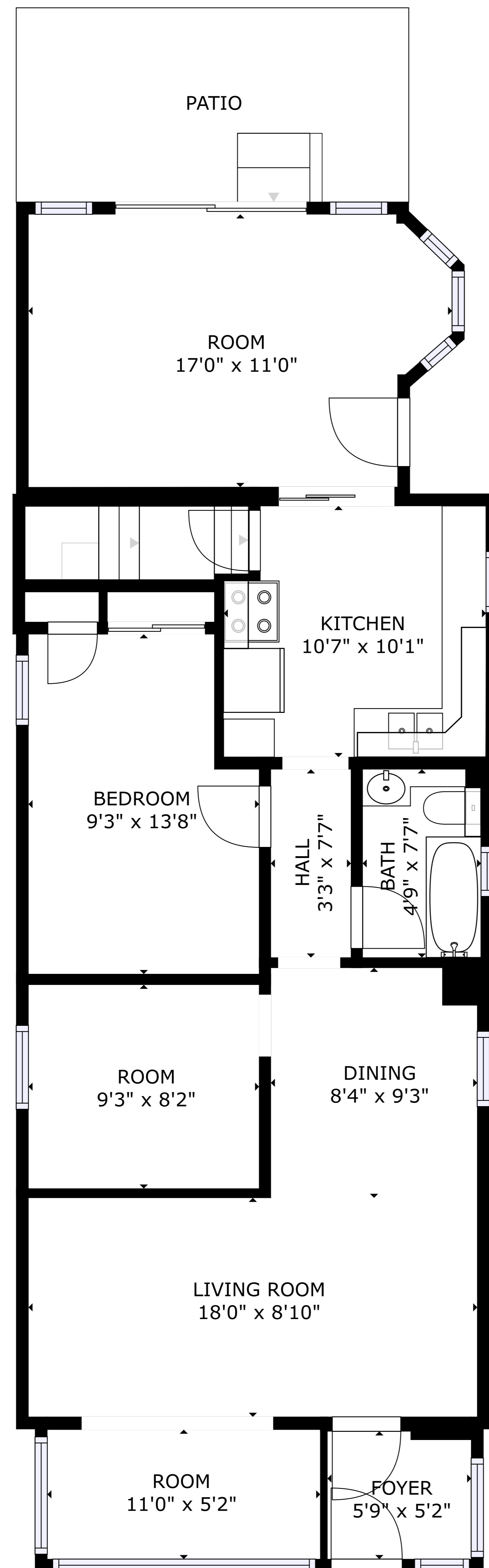
Main Level
