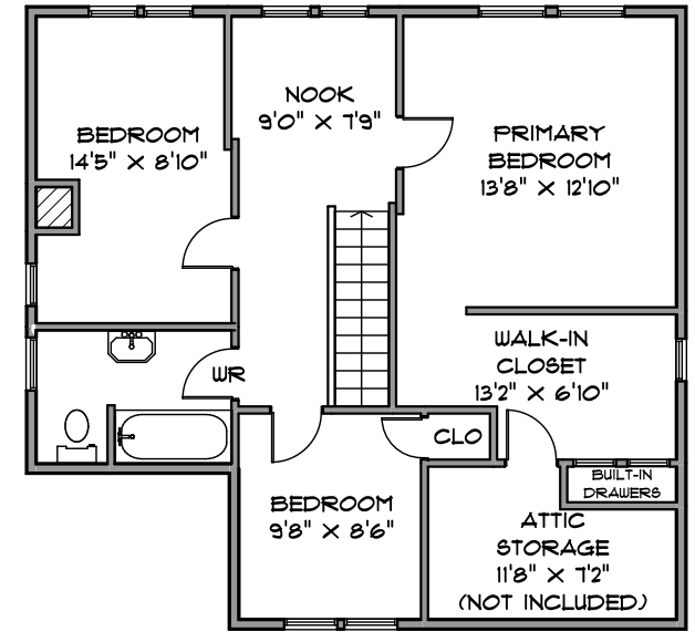
UPPER LEVEL 761 SQ. FT.
