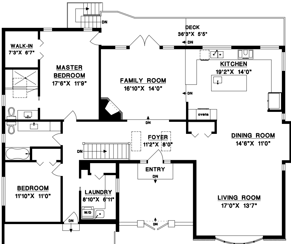
MAIN LEVEL
