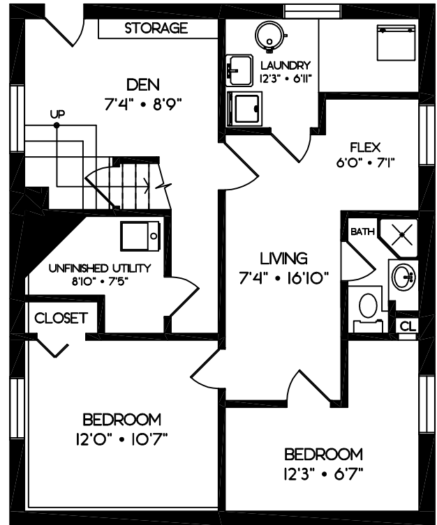
LOWER FLOOR: FINISHED AREA: 832 SQFT UNFINISHED AREA: 54 SQFT
