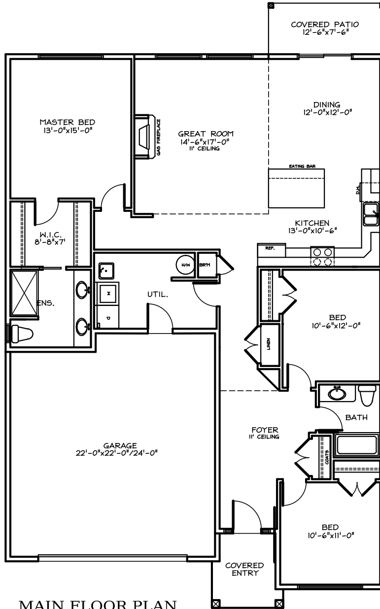
MAIN FLOOR PLAN 1705 SQ. FT.
