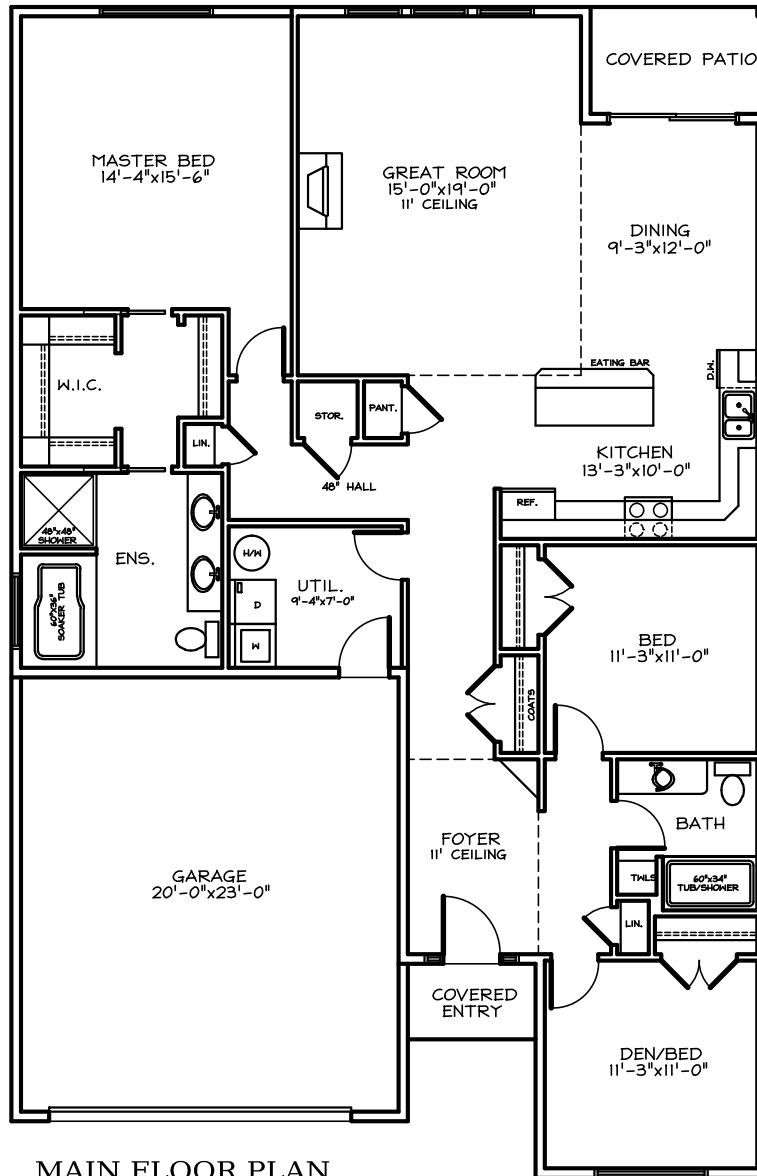
MAIN FLOOR PLAN 1802 SQ. FT.
