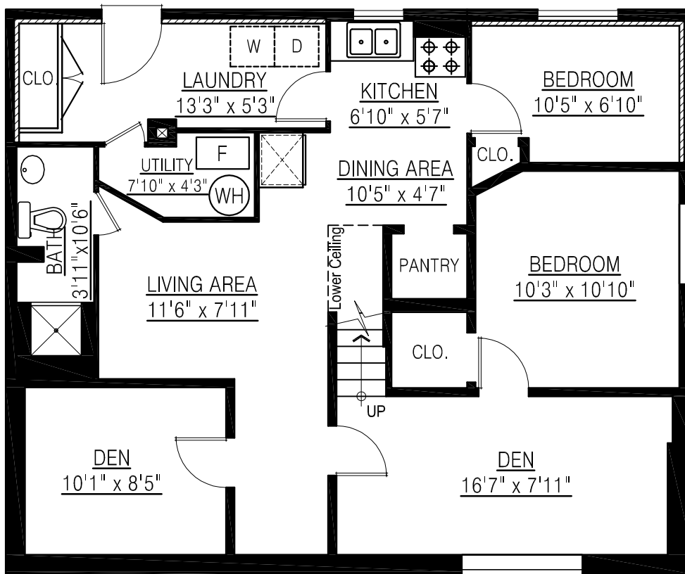
BASEMENT FLOOR PLAN FLOOR AREA: 977 sq.ft.
