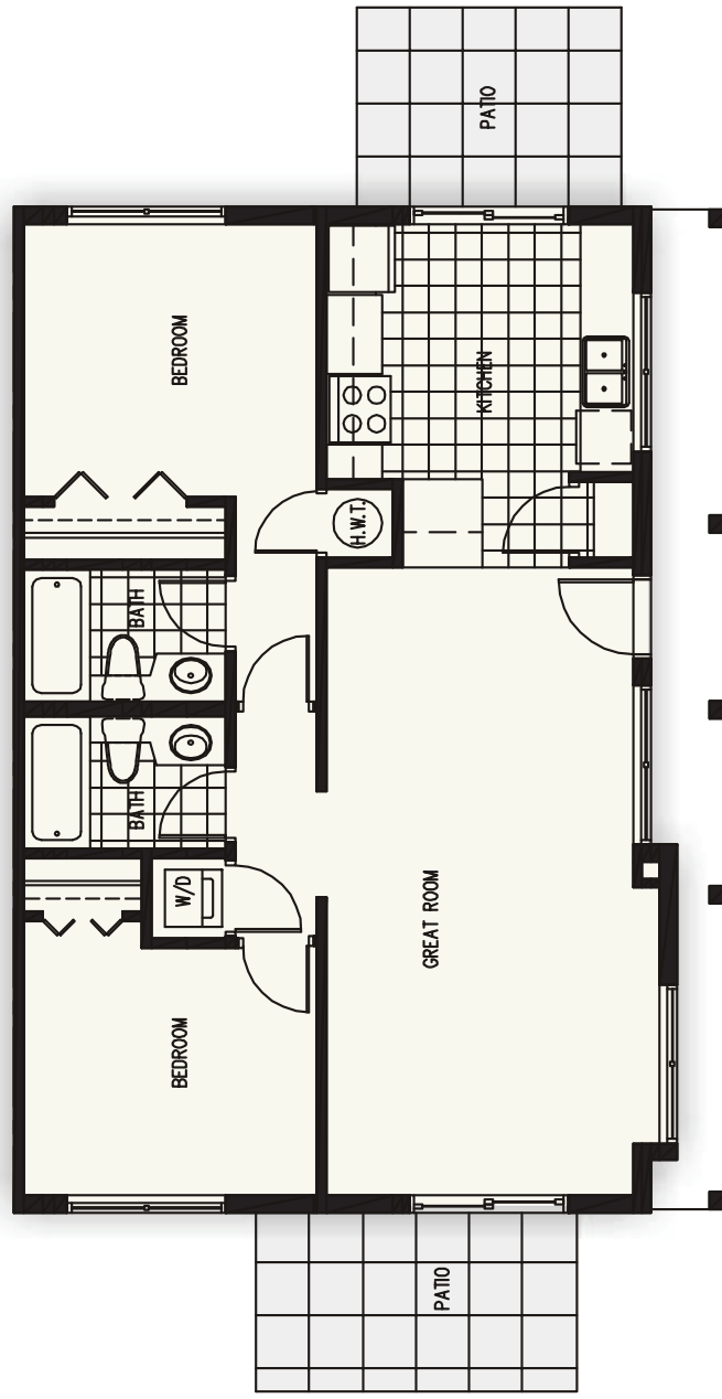
GROUND FLOOR
