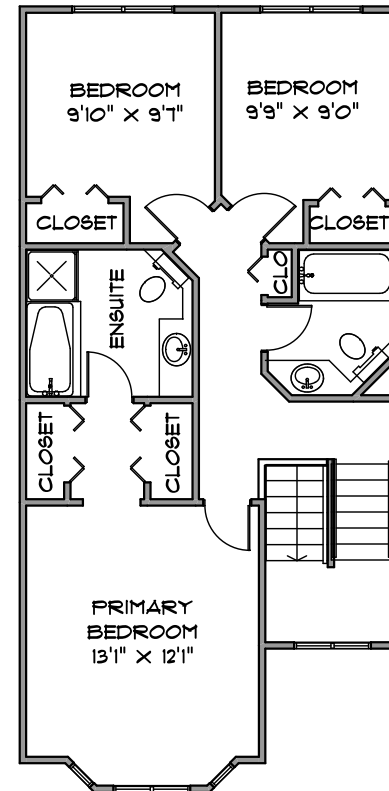
UPPER LEVEL 751 SQ.FT.
