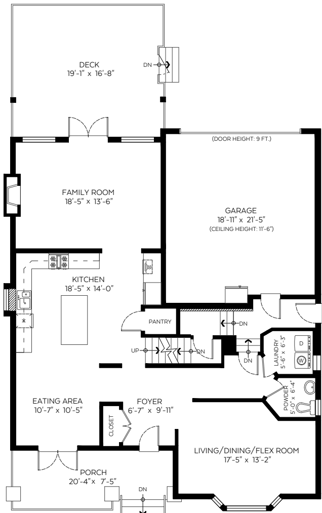
Main Floor Plan Floor Area: 1,279 sq.ft. Ceiling Height: 9 ft.
