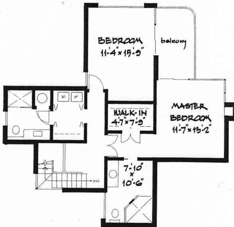
UPPER FLOOR
