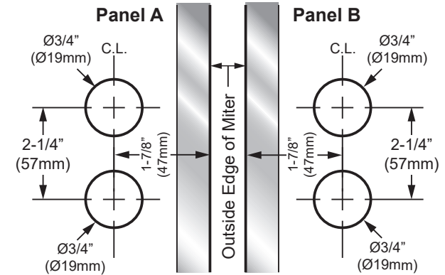
45° Mitered Glass Glass Thickness: 1/2" (12mm)
