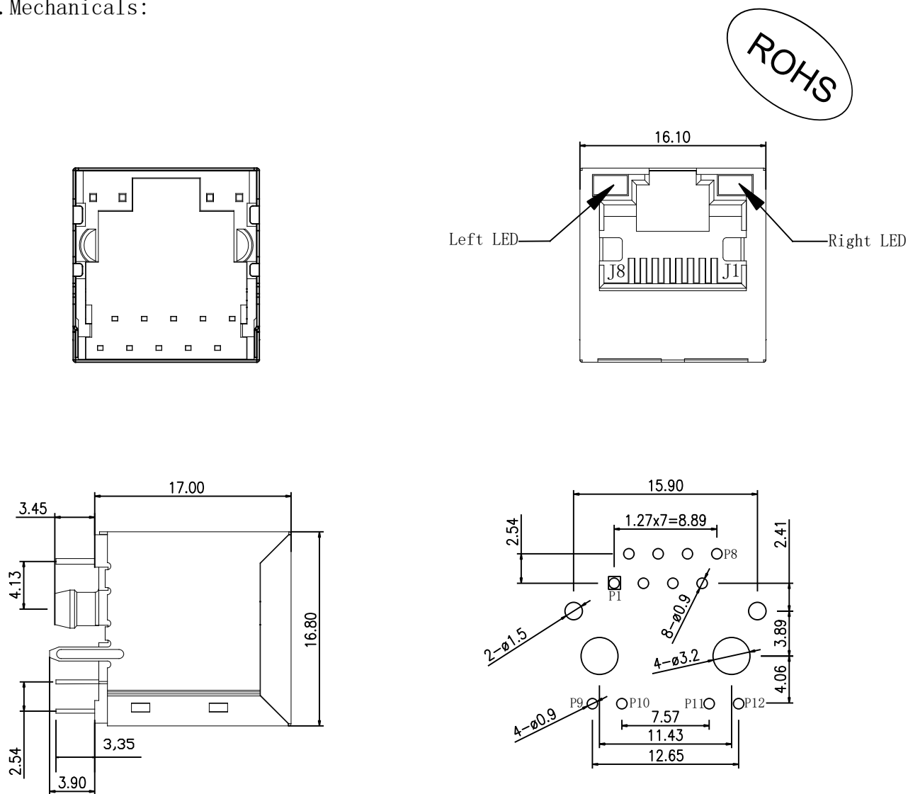
P. C. B RECOMMENDED HOLE LAYOUT SEEN FROM COMPONENT SIDE. ALL CENTERLINE DIMENSIONS ARE BASIC *Specification subject to change without notice
