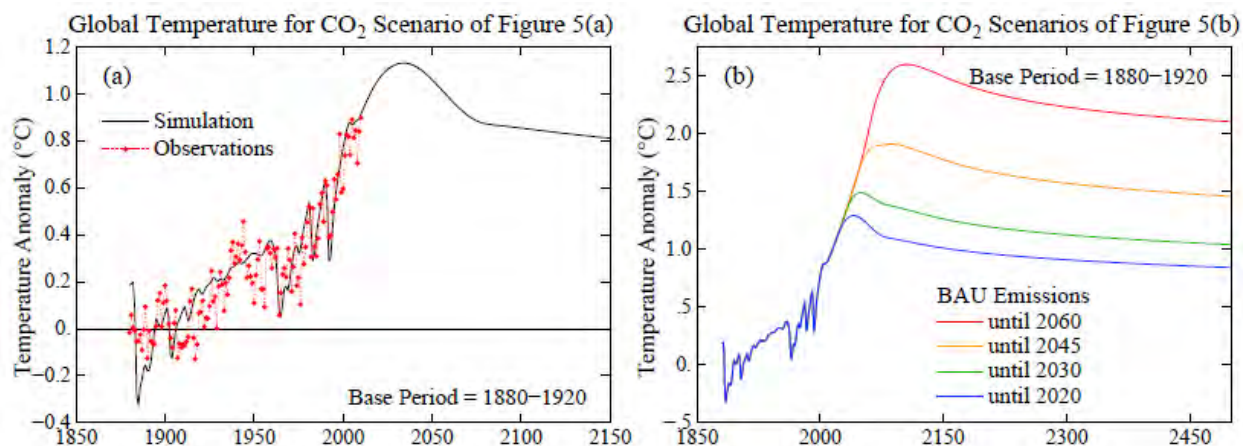
Figure 6. Simulated future global temperature for the CO 2 scenarios of Figure 5. Observed temperature record is from Hansen et al. (2010). Temperature is relative to the 1880-1920 mean. Subtract 0.26°C to use 1951-1980 as zero-point. Subtract 0.70°C to use 5-year running mean in 2000 as zero point.
