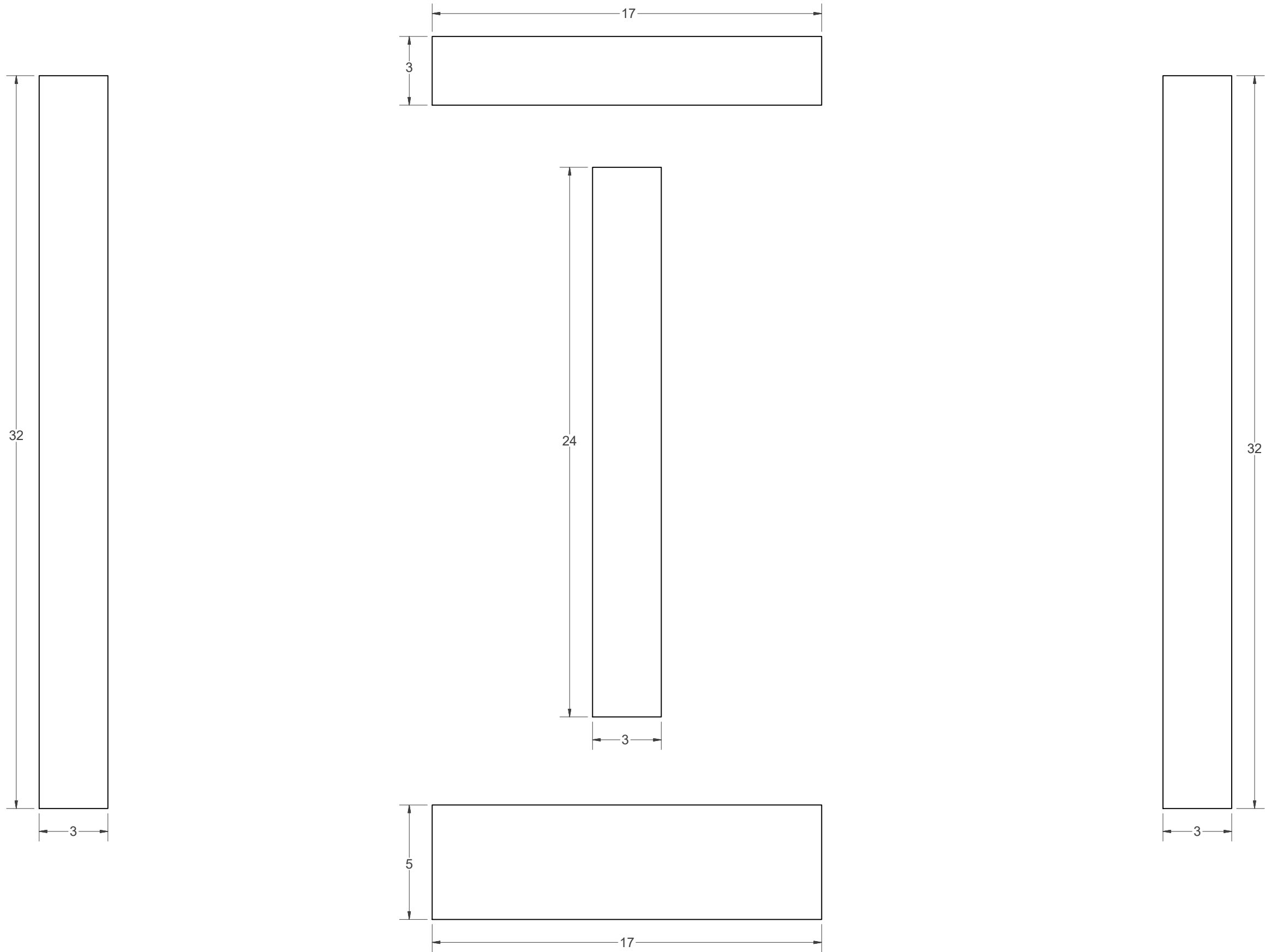
END PANEL OVERLAY STRIPS (ALL 1/2 POPLAR)
