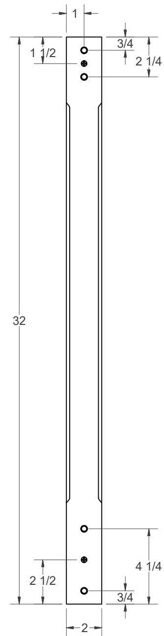
END PANEL (END VIEW)
