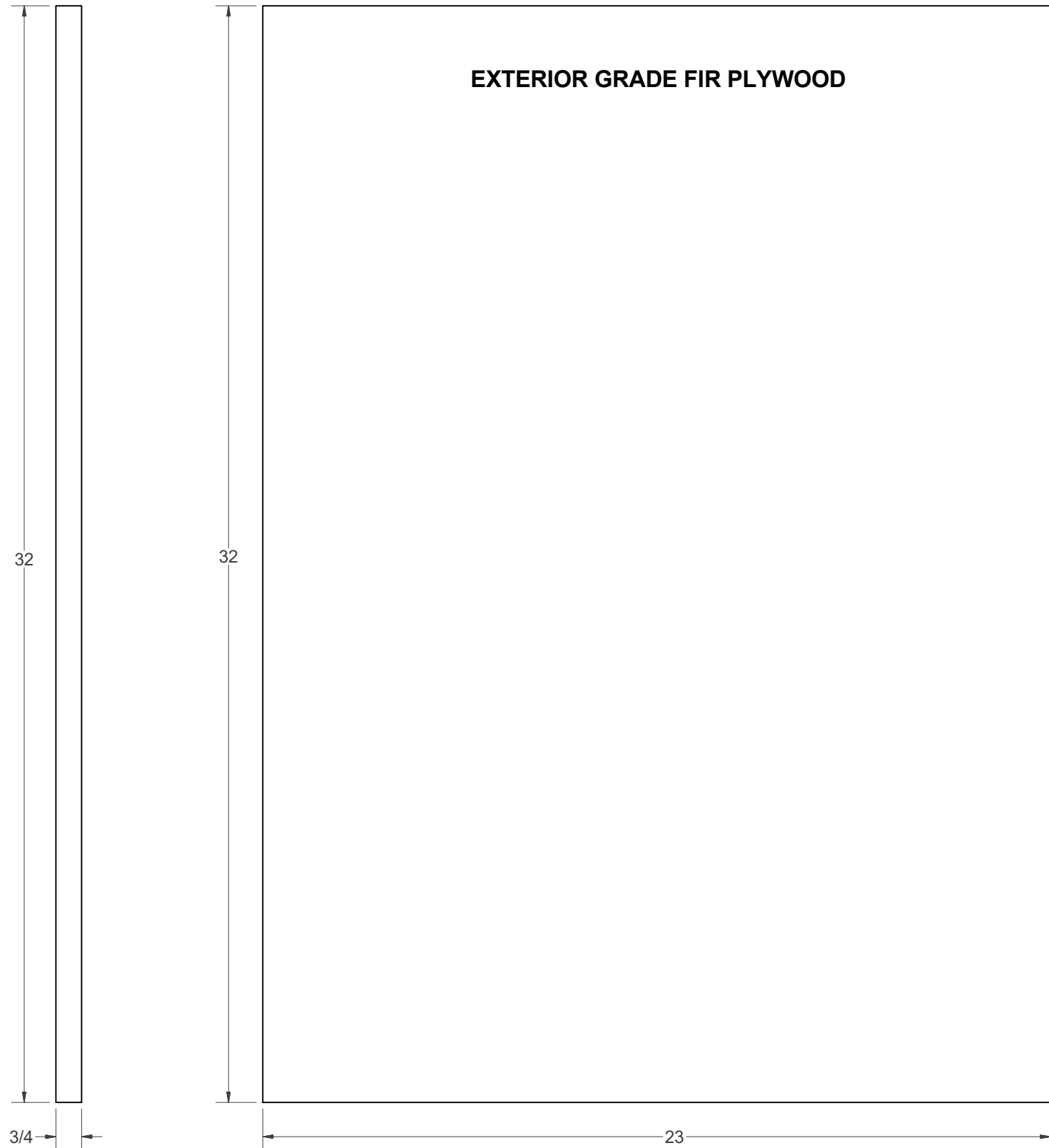
SIDE PANEL (NEED 4)
