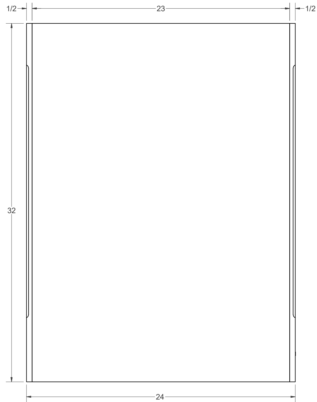
END PANEL (INSIDE VIEW)
