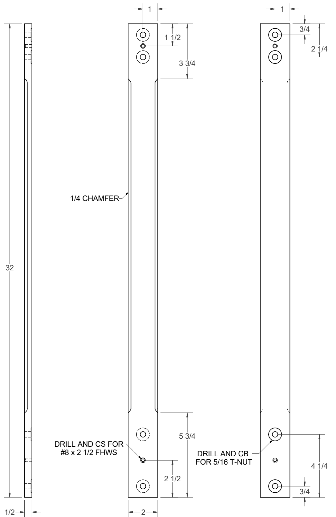
SIDE PANEL ASSEMBLY-FRONT STILE (NEED 4)
