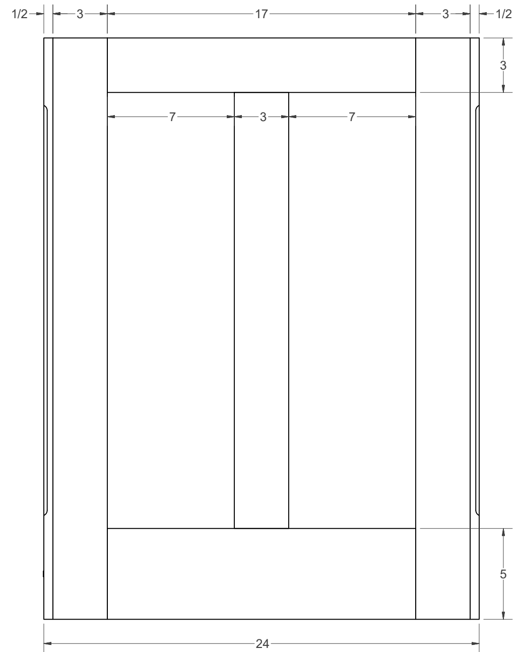
END PANEL (OUTSIDE VIEW)
