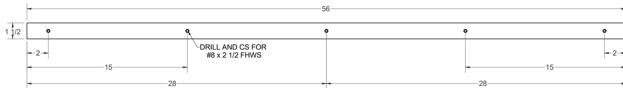
BOTTOM SHELF CLEAT
