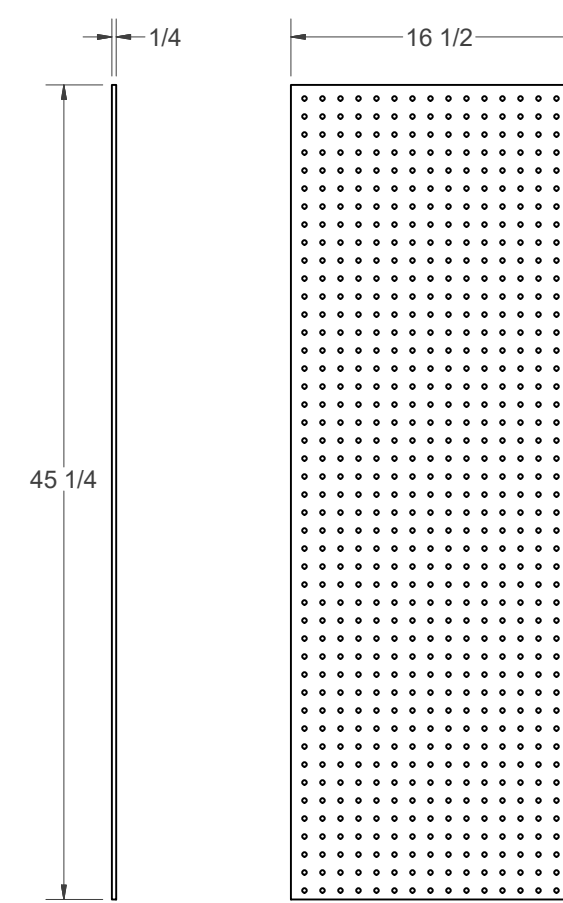
PEGBOARD
