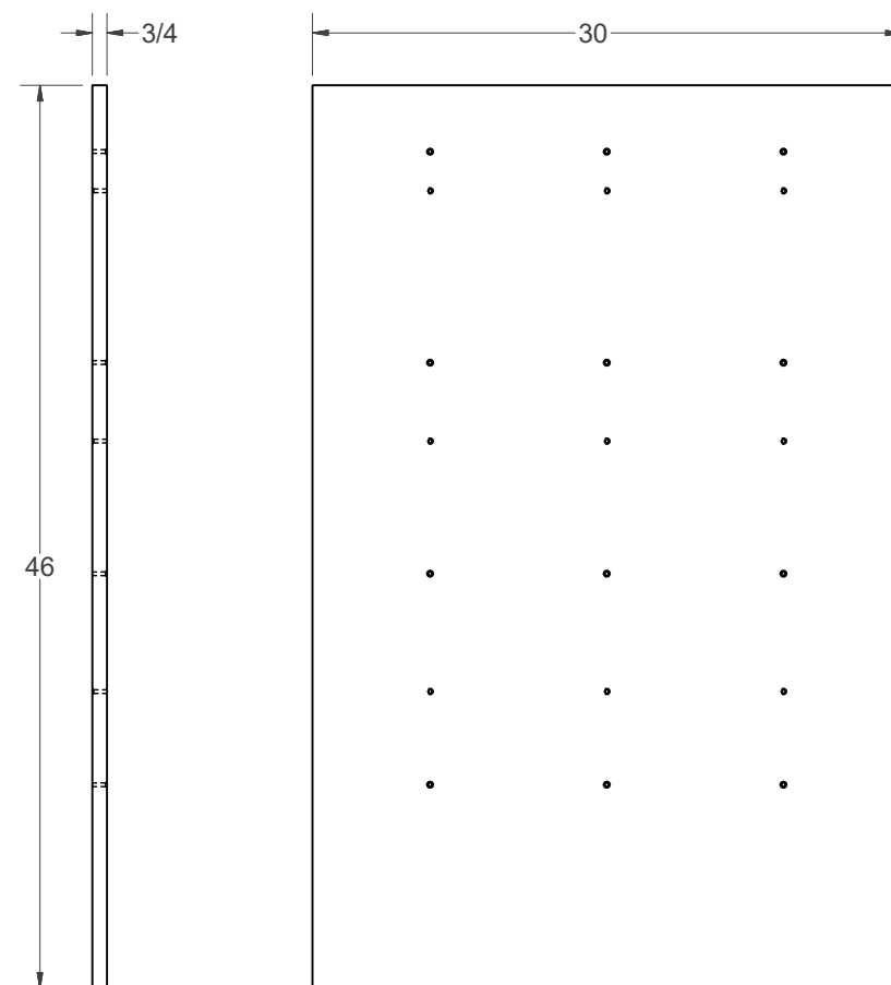
CENTER PANEL
