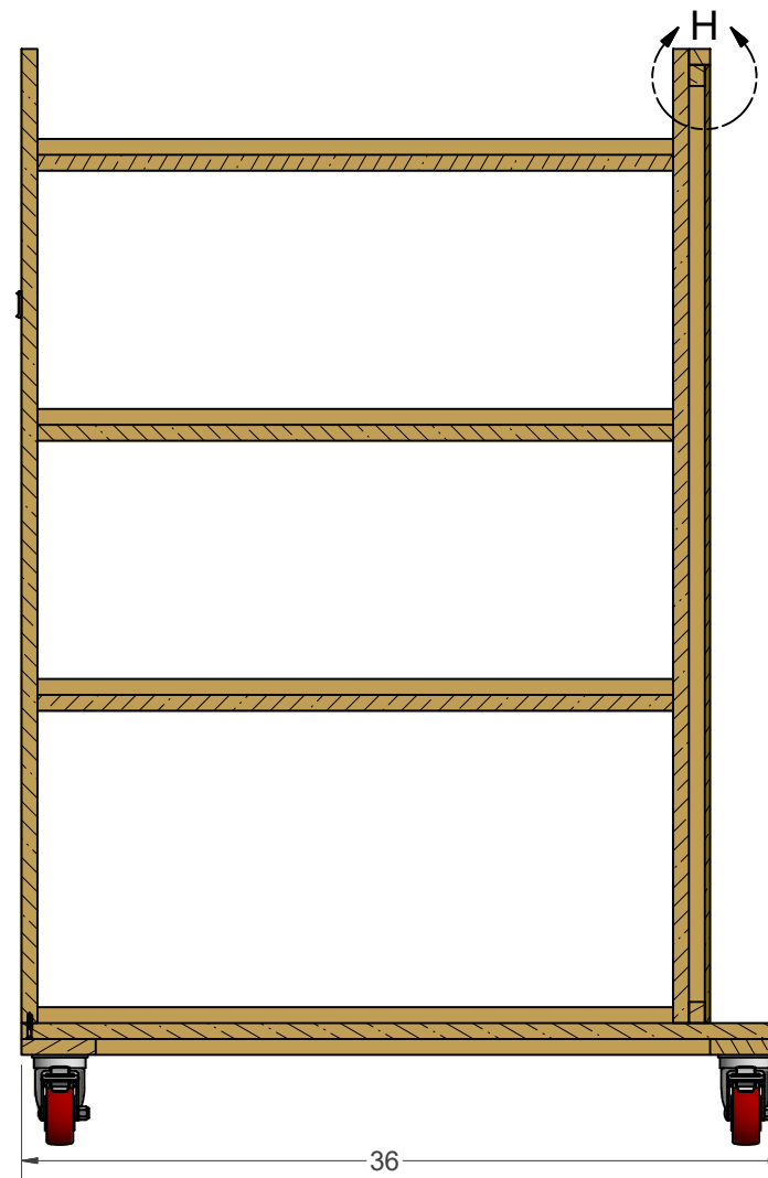
SECTION F-F
