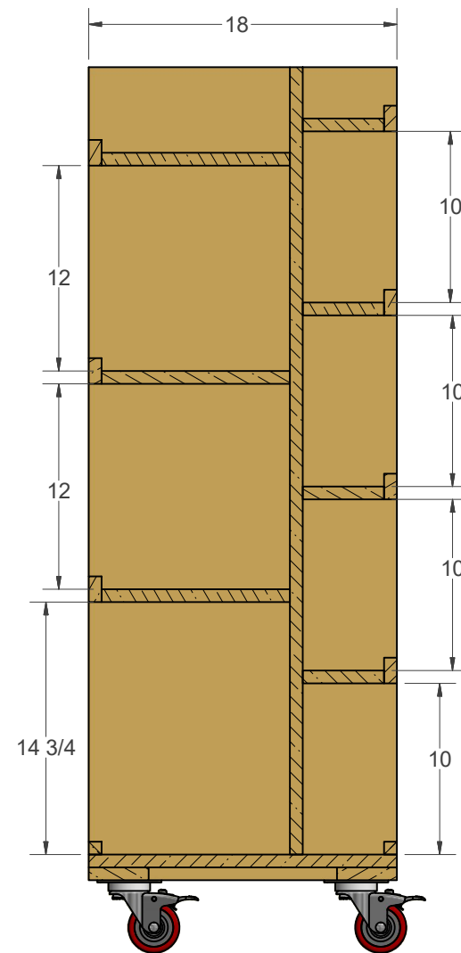
SECTION E-E
