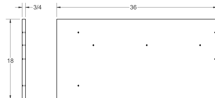
BASE
