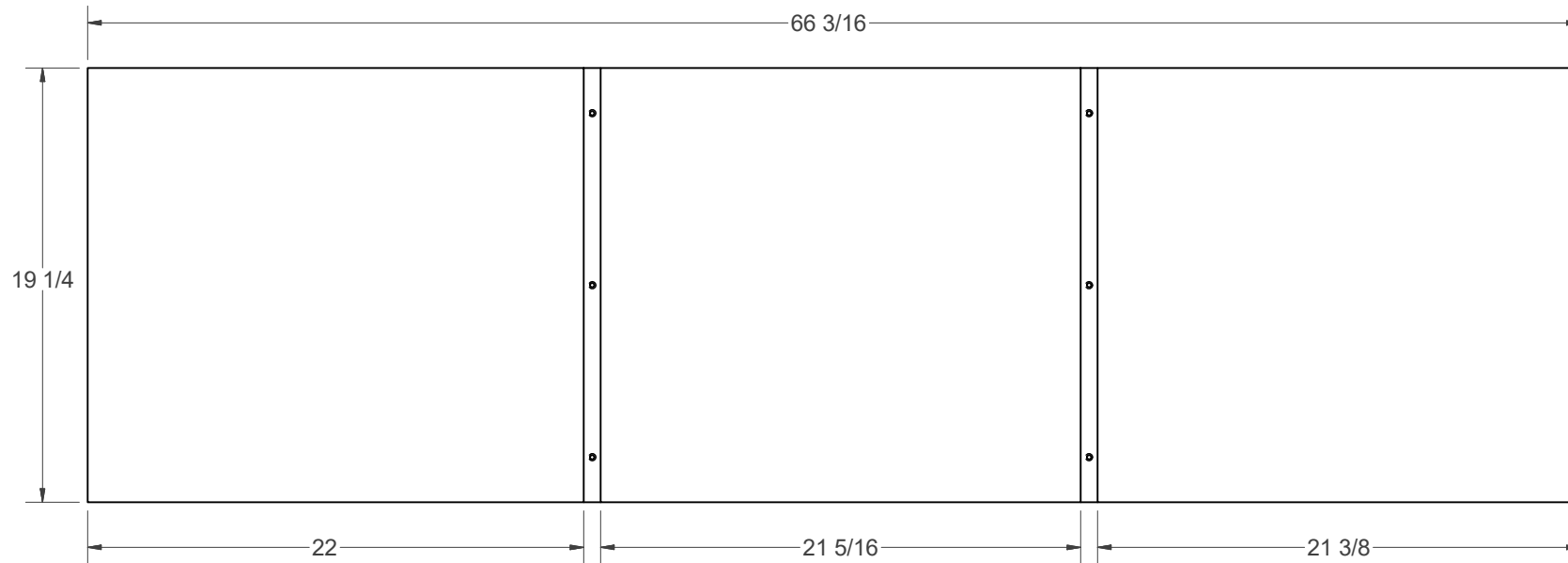
BASE BOX TOP PANEL
