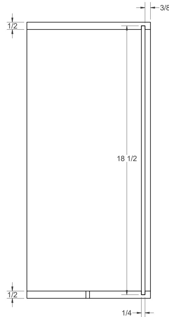
DRAWER FRONT TRIM (CROSS SECTION)
