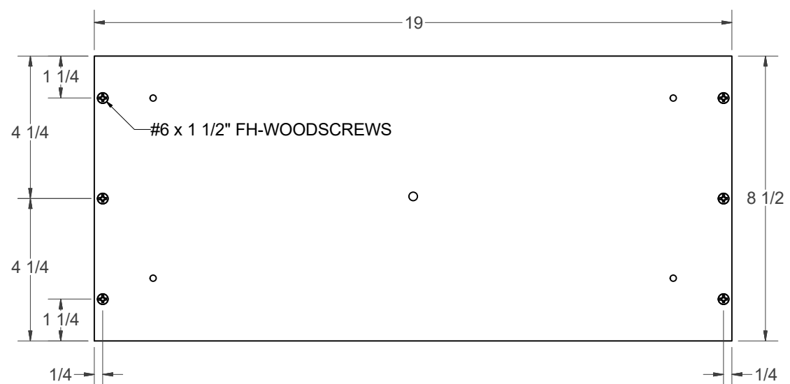
DRAWER BOX (FRONT VIEW)
