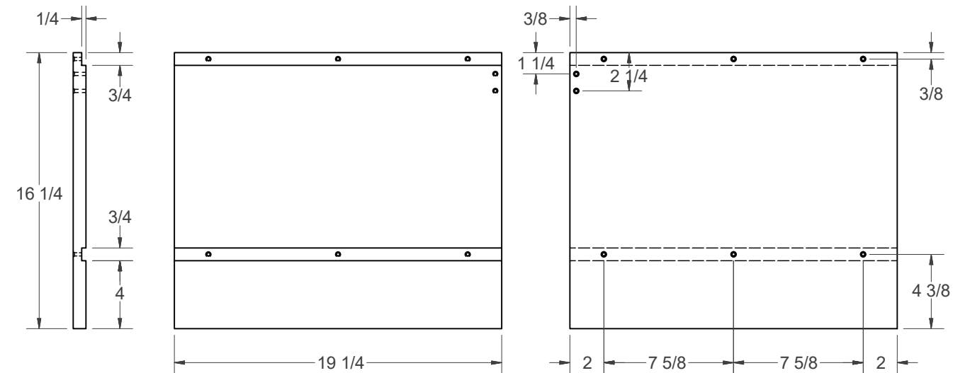
BASE BOX END PANEL (NEED 2 FOR EACH UNIT)
