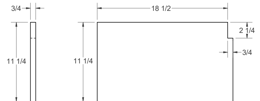
DIVIDER PANEL (NEED 2 FOR EACH UNIT)
