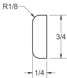
SEAT EDGING (12'-0" LONG)
