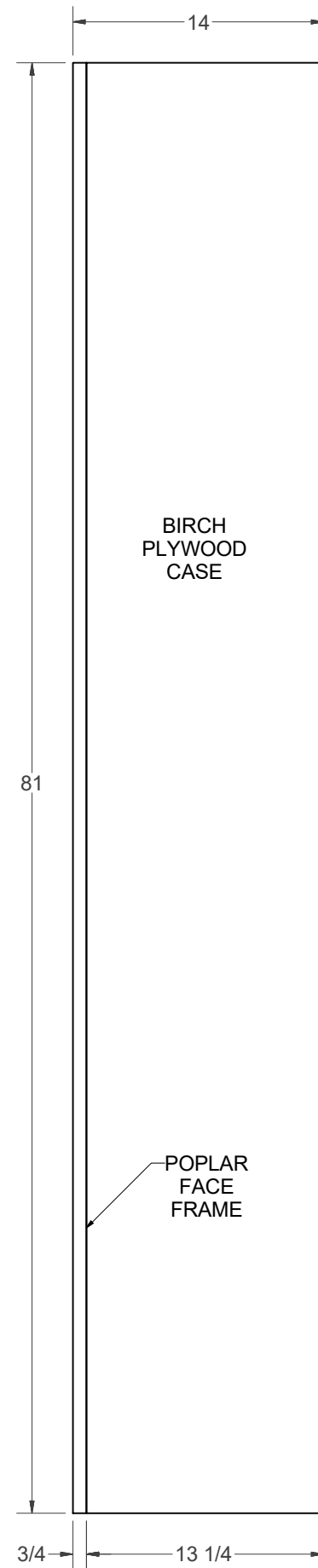
SIDE VIEW
