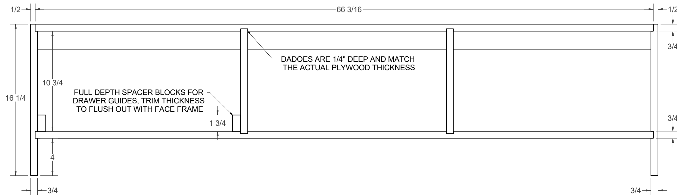
BASE BOX (LEFT)
