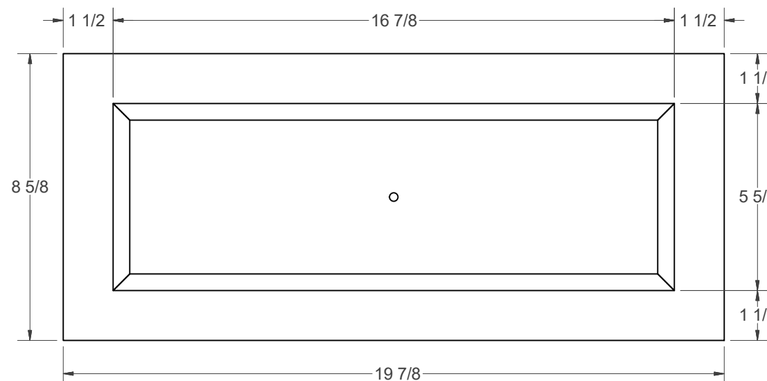
DRAWER FALSE FRONT
