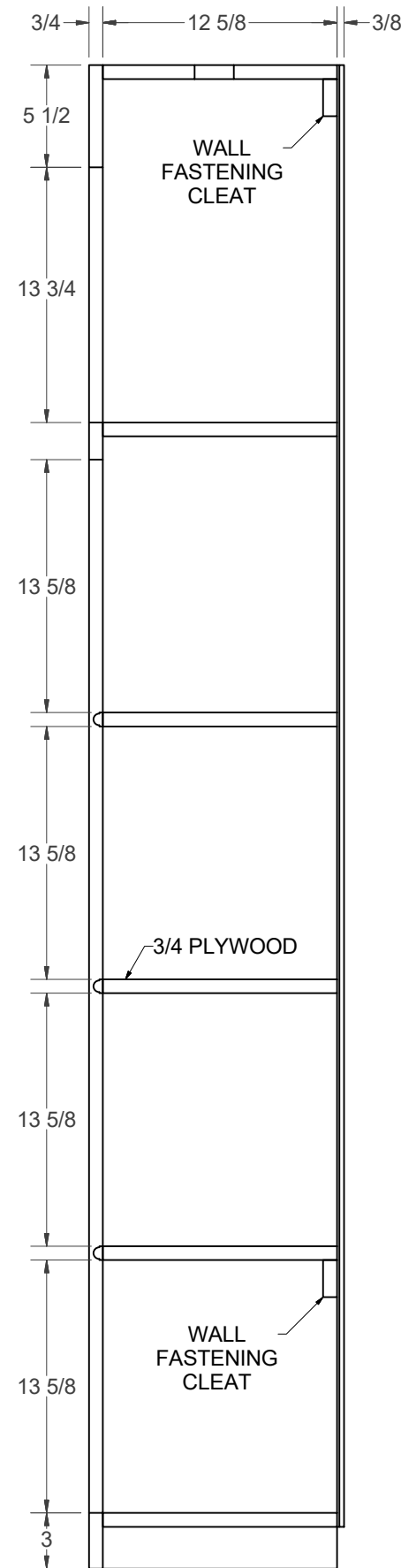
SECTION VIEW
