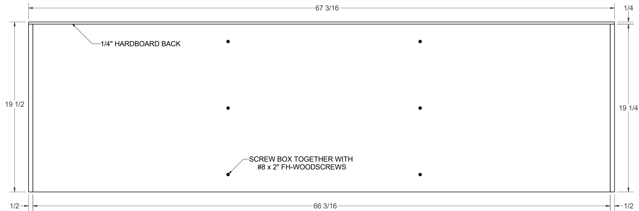
TOP VIEW
