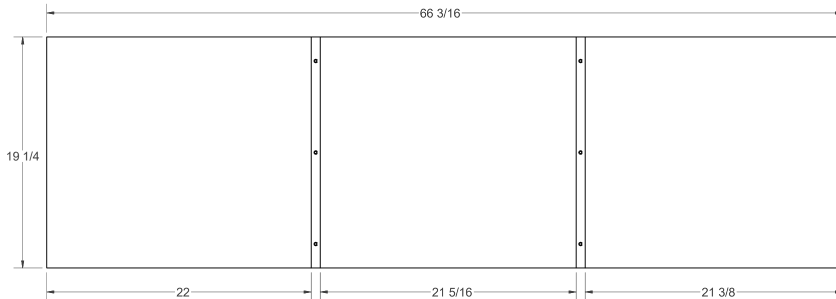
BASE BOX BOTTOM PANEL
