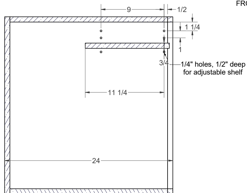
SIDE VIEW
