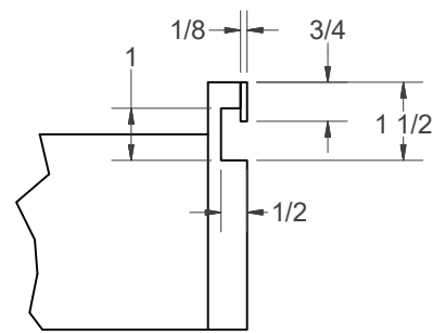
DETAIL L SCALE 1 / 2
