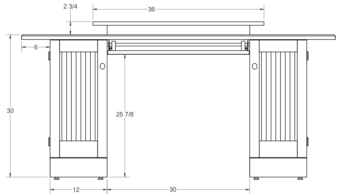
Front View
