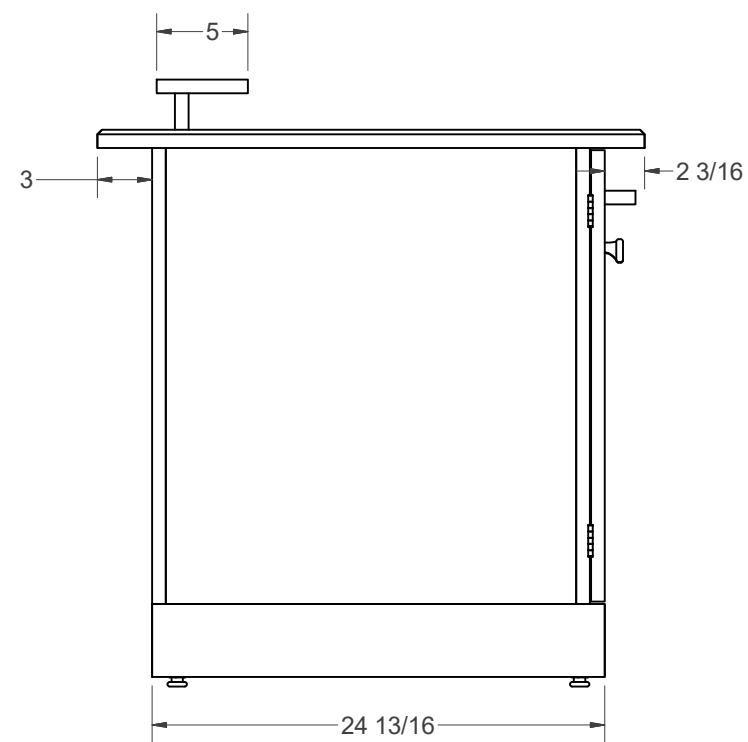
End View
