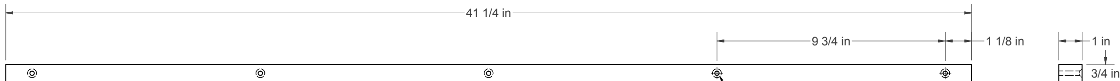
(E) - CLEATS (MAKE FOUR)
