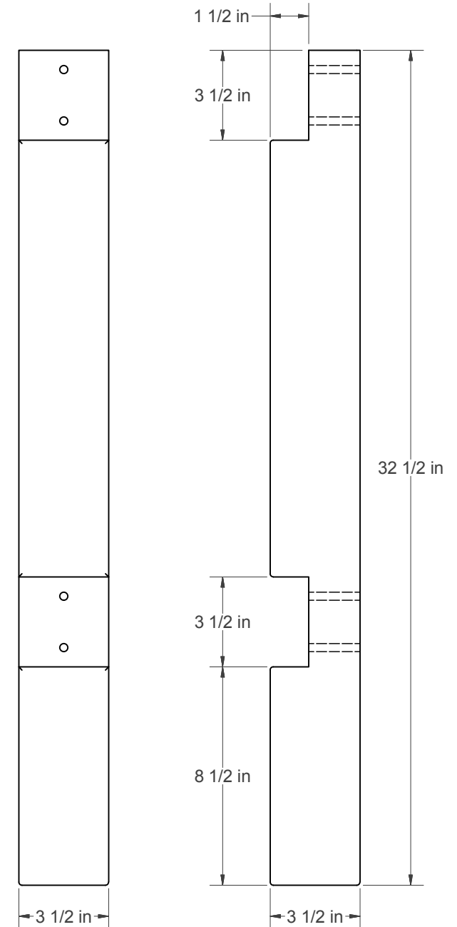
(A) - LEGS (MAKE SIX)
