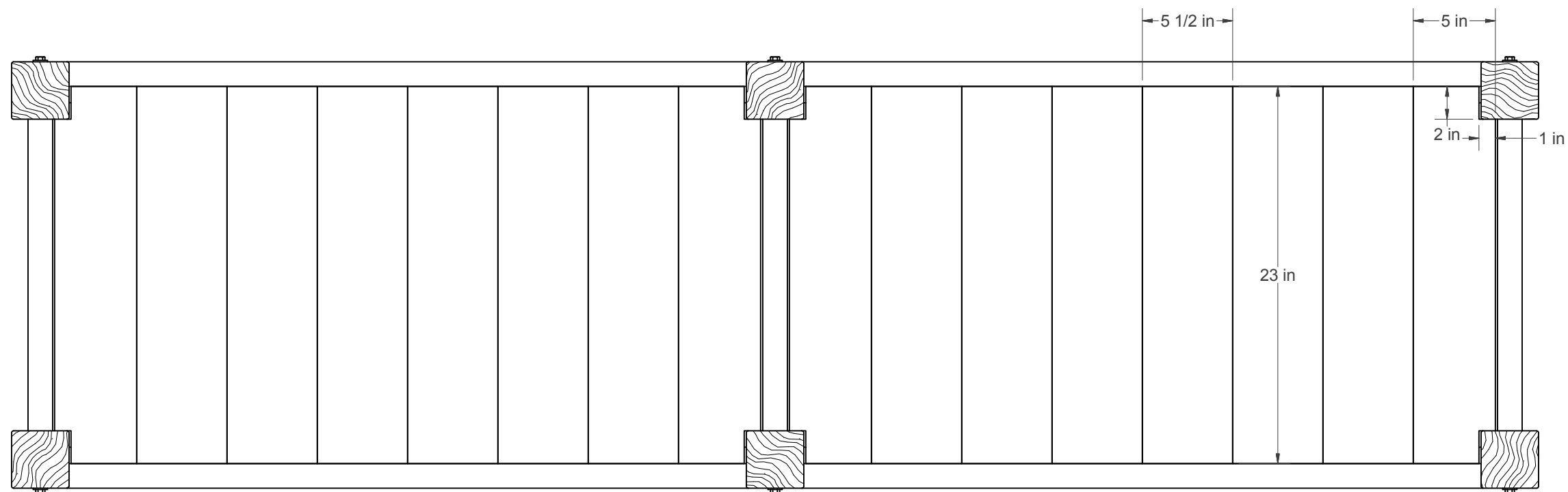
(F) - SHELF SLATS (NEED 16)
