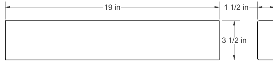
(C) - SHORT CROSS RAILS (MAKE SIX)
