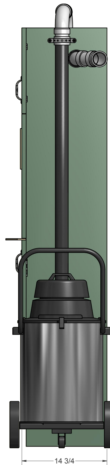
SIDE VIEW
