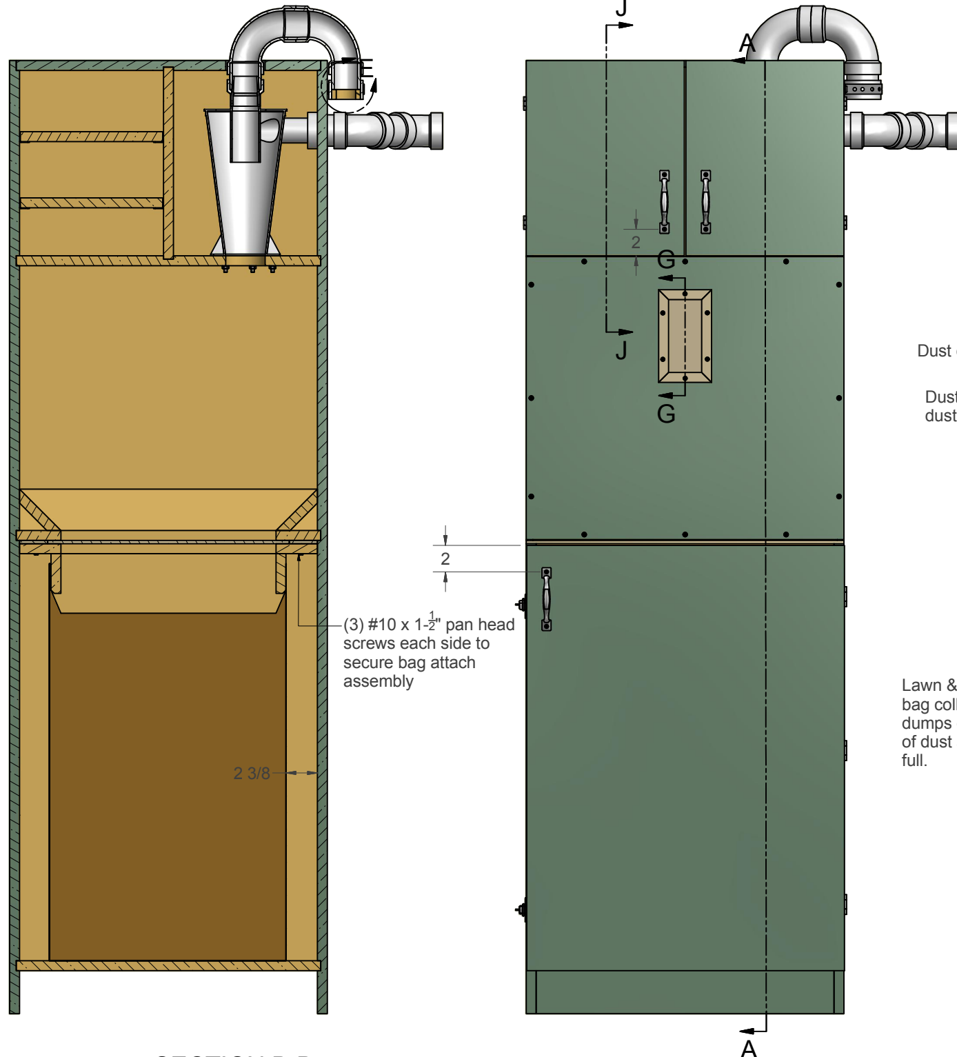
SECTION B-B
