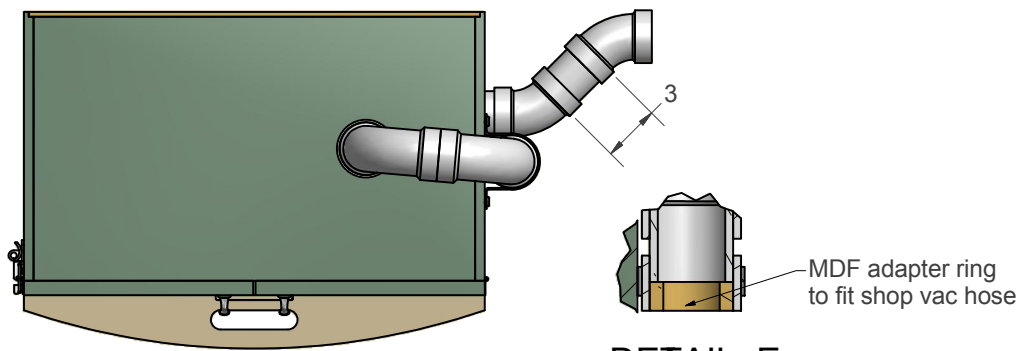
DETAIL E
