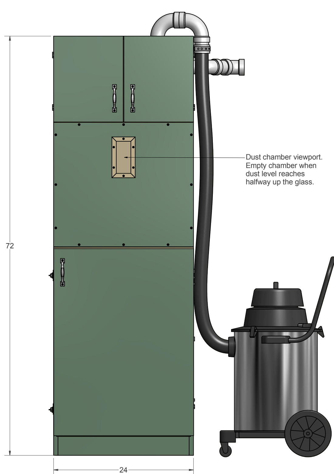
FRONT VIEW
