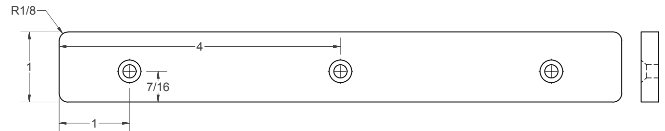
I - STOPS (2)
