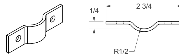
(W) - NOSE CLAMP
