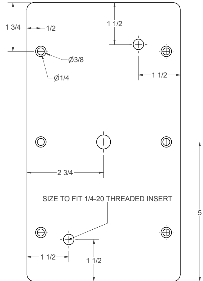
(K) - Y-AXIS PLATFORM
