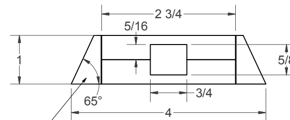
(F) - X-AXIS WAY (2 PCS)
