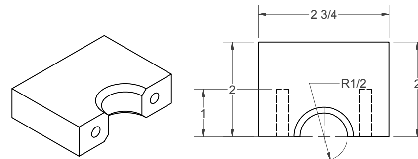
(S) - NOSE BRACKET
