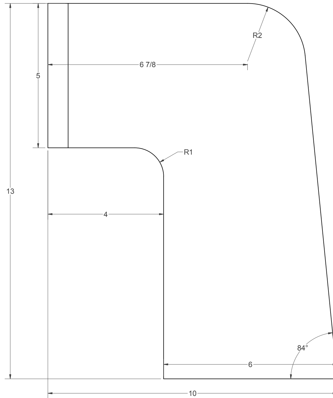
(B) - POST - LEFT & RIGHT MIRRORED (2 LAYERS 3/4" PLY)
