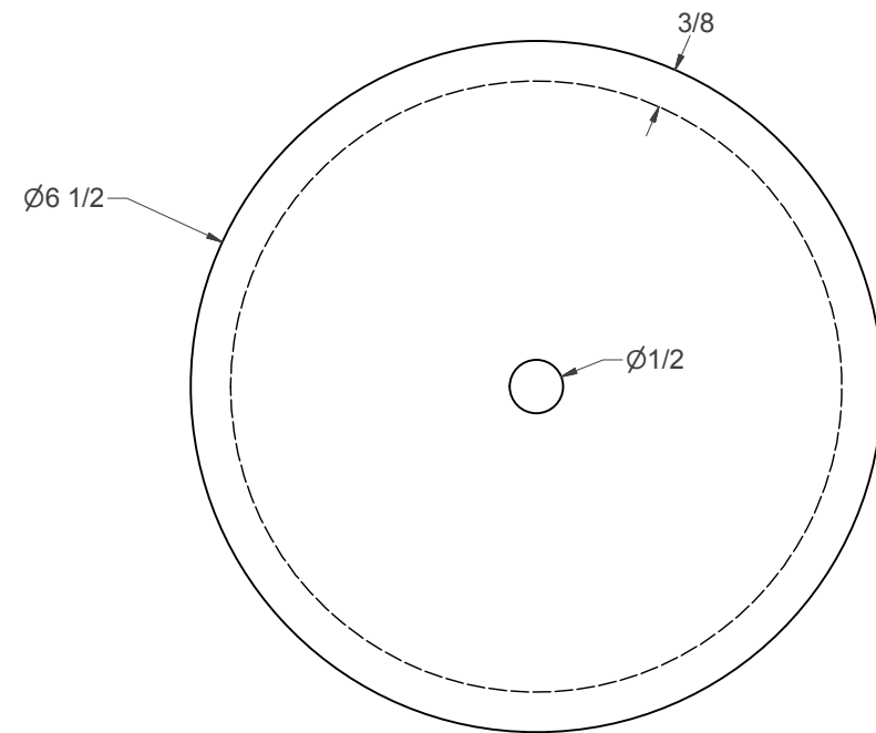
(M) - ROTATING TABLE BASE
