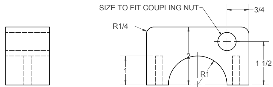
(R) - TOOL BRACKET
