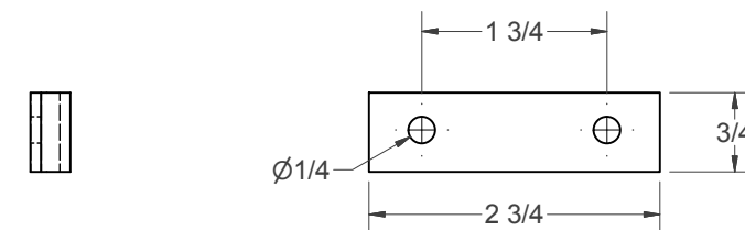
(W) - NOSE CLAMP
