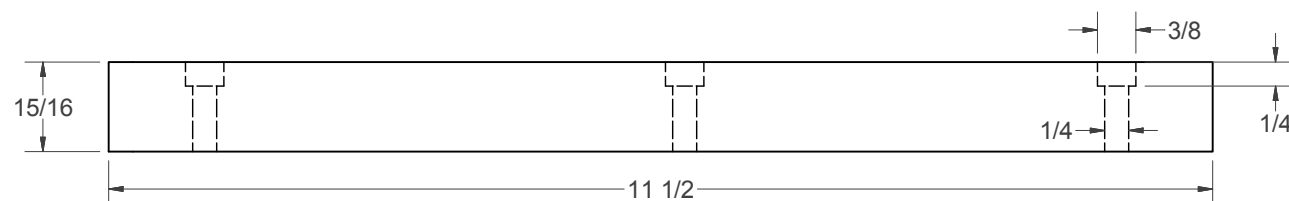
(H) - X-AXIS GIBB (2 PCS)
