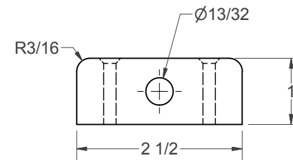
(G) - END BLOCK (2 PCS)
