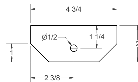
RISER BLOCK (NEED 2)
