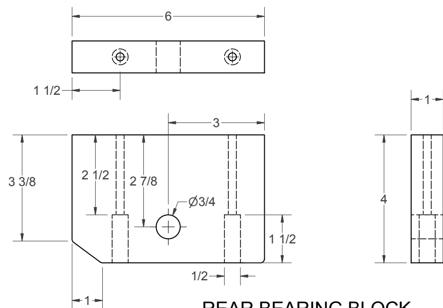
REAR BEARING BLOCK
