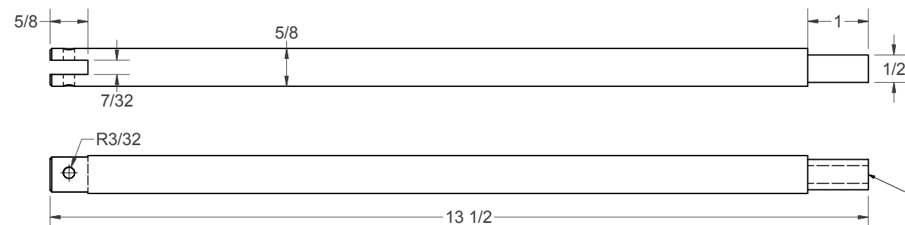
LOCKING SHAFT
