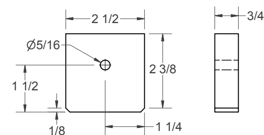
STOP BLOCK
