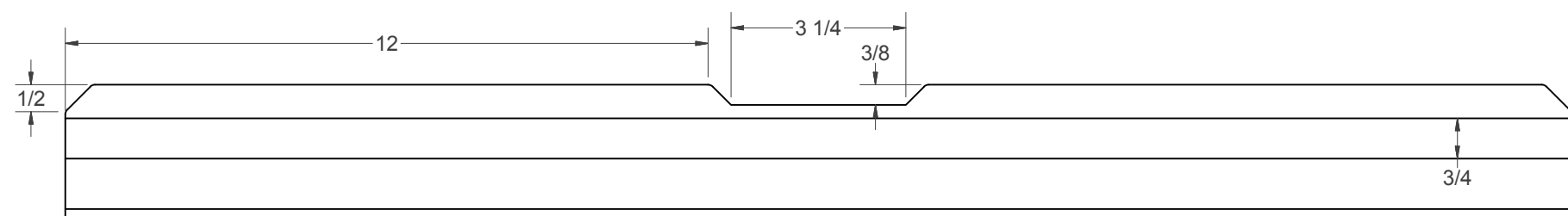
FENCE FACE
