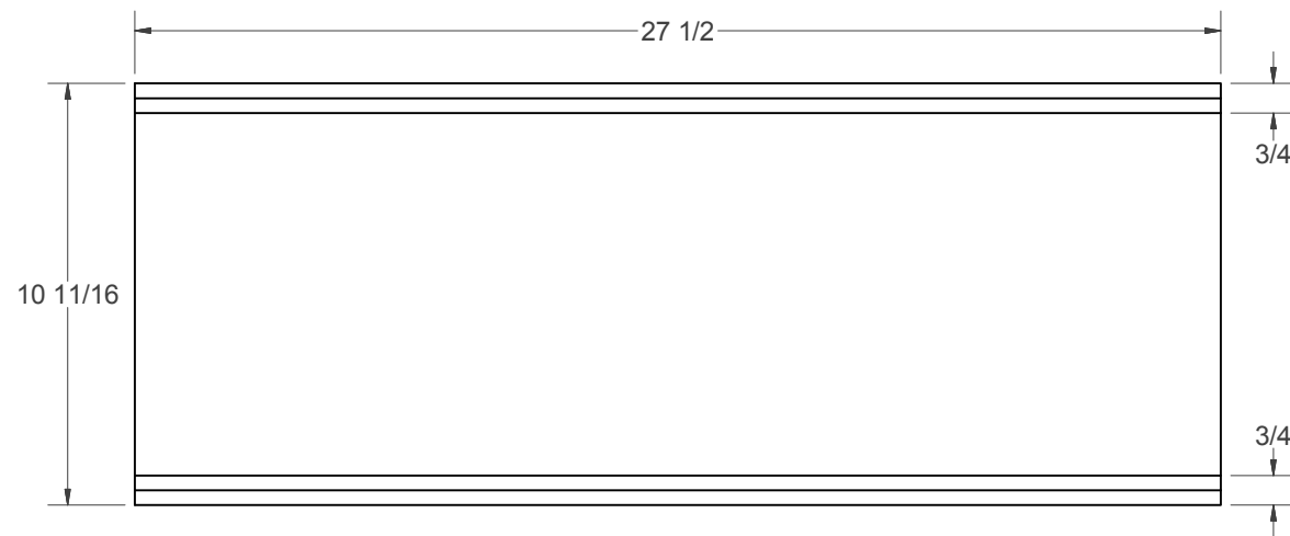
(M) - CASE SIDE (RIGHT)
