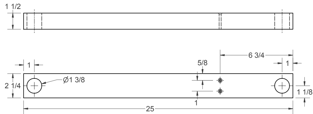
(G) - HANDLE RAIL
