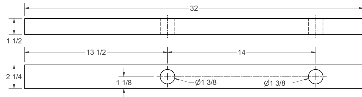
(H) - OUT-FEED SUPPORT RAIL
