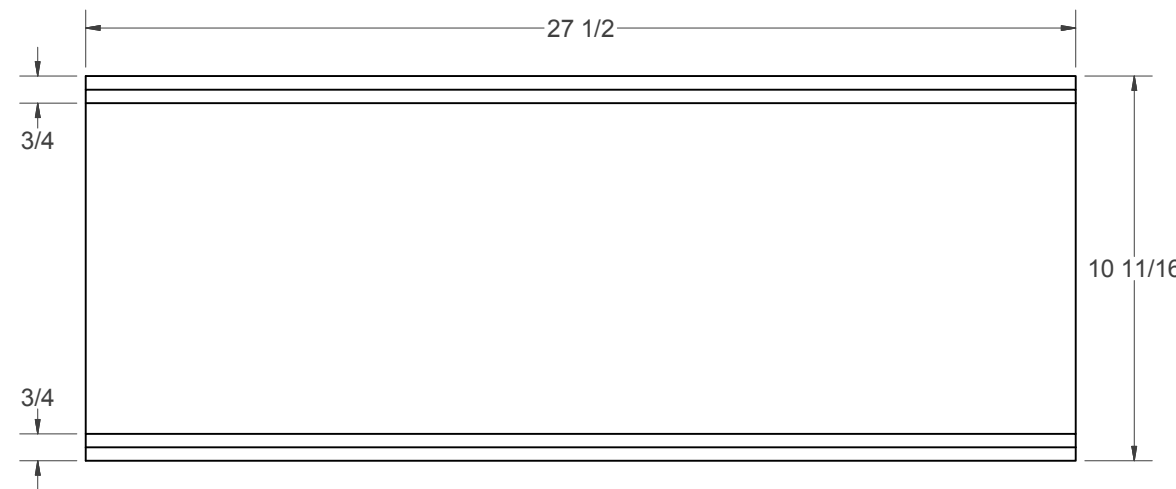
(M) - CASE SIDE (LEFT)
