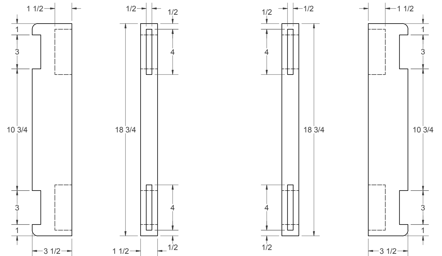
(B) - RIGHT STILE (NEED 2)
