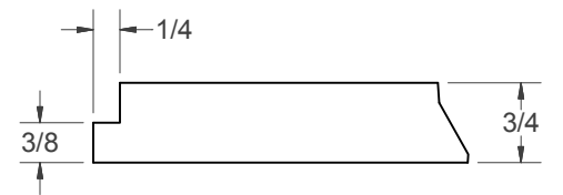
CASE JOINERY RABBET
