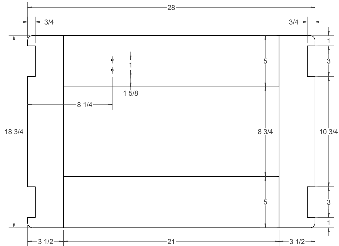
RIGHT END FRAME
