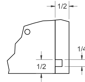
DRAWER BOTTOM DETAIL
