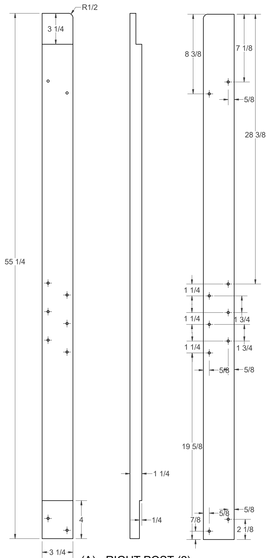
(A) - RIGHT POST (2)
