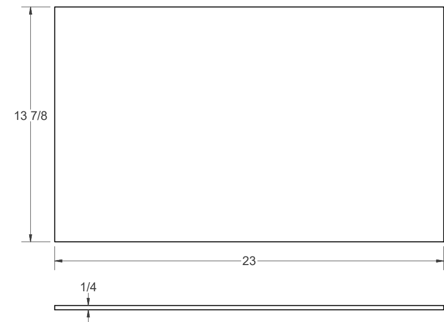
(L) - LOWER DRAWER BOTTOM (1)
