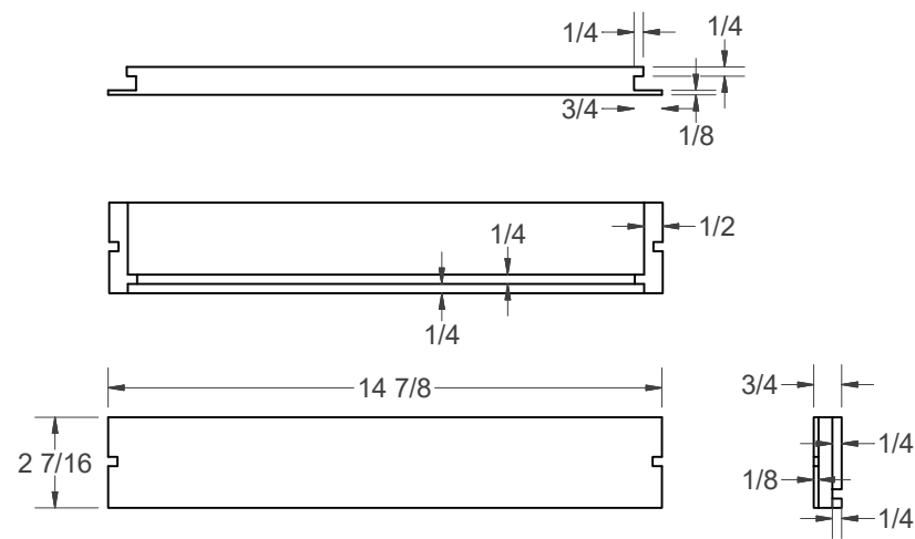
(J) - DRAWER FRONT/BACK (2)
