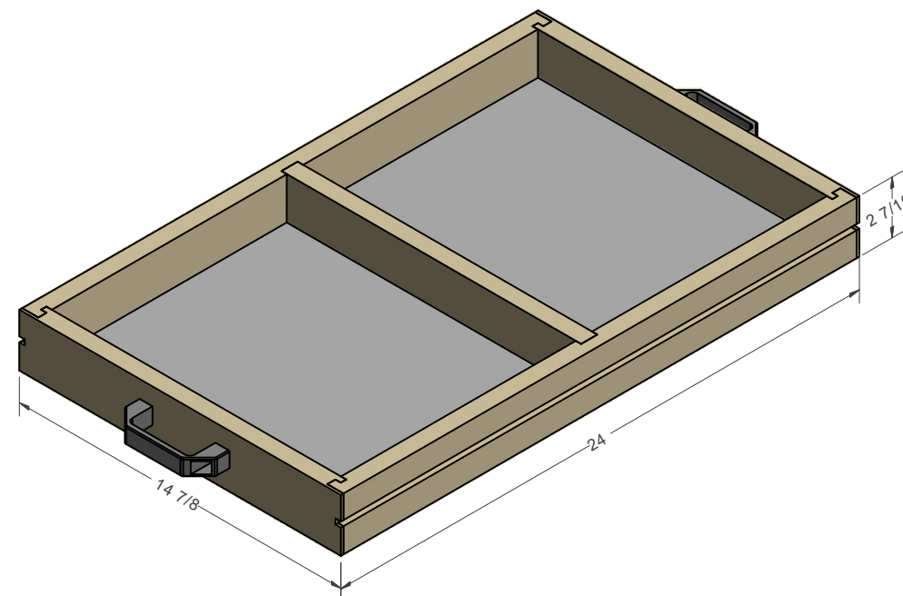
NARROW DRAWER (1)
