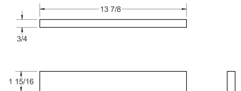
(K) - LOWER DRAWER DIVIDER (1)
