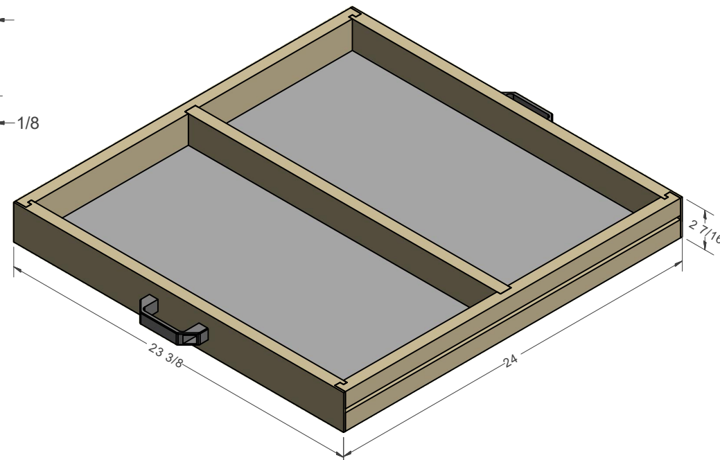
WIDE DRAWER (2)
