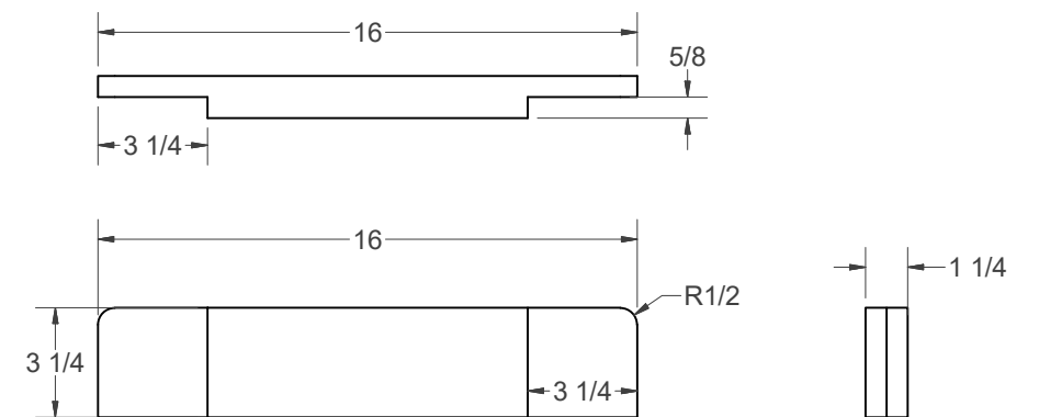
(B) - RAIL (2)
