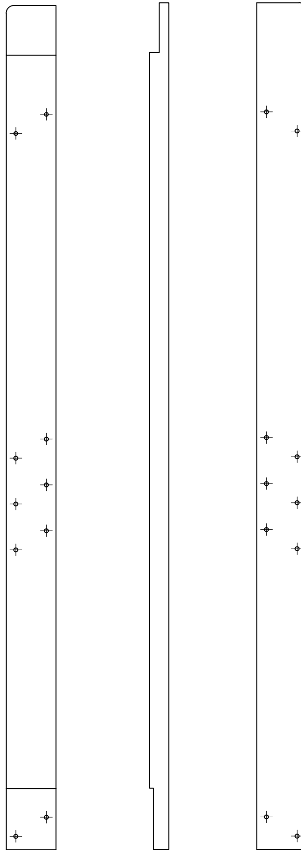
(A) - LEFT POST (2)
