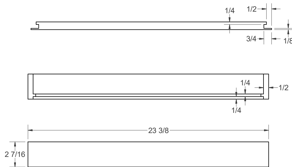
(M) - DRAWER FRONT/BACK (4)
