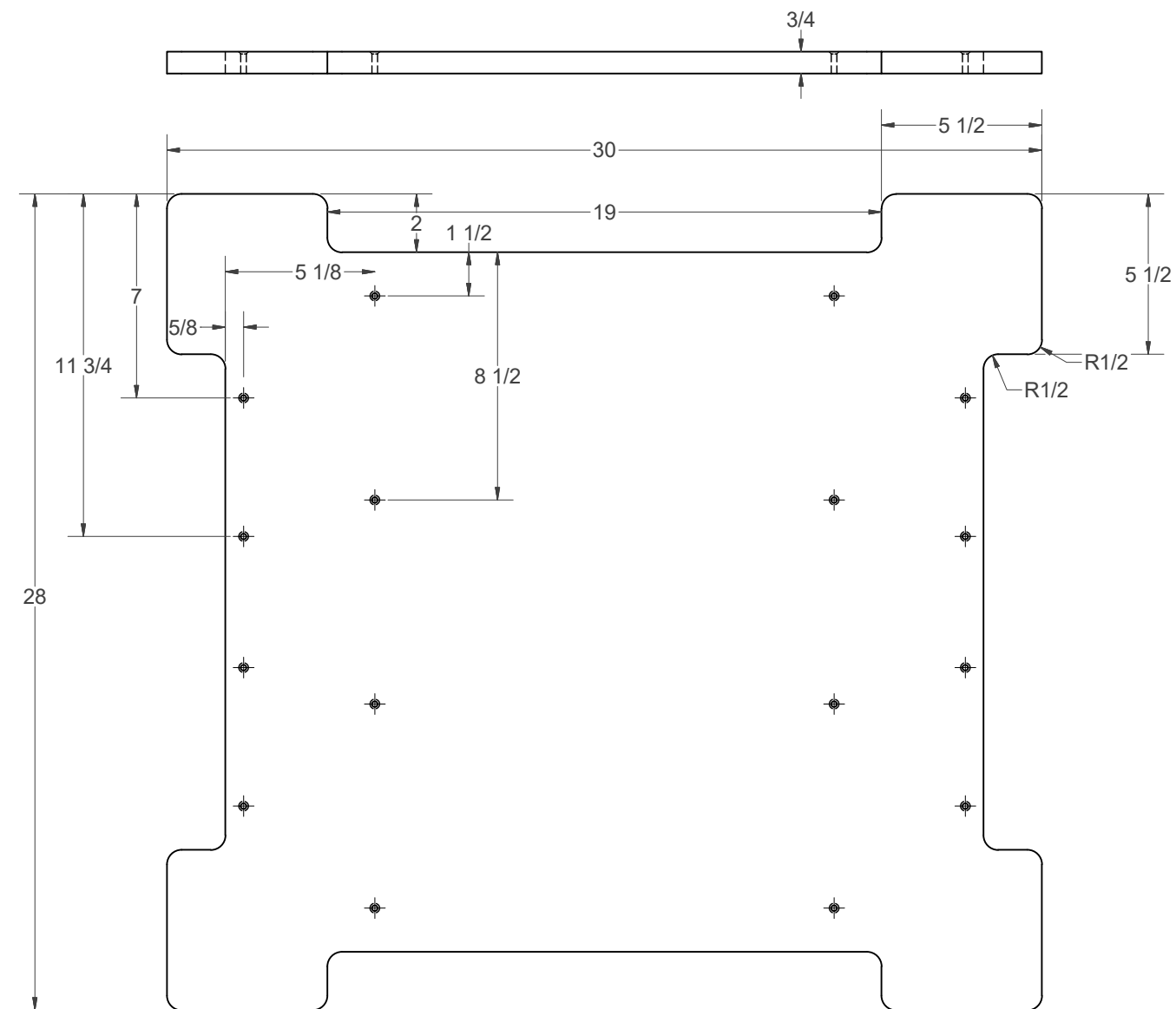
(C) - BASE - 1 1/2" THICK
