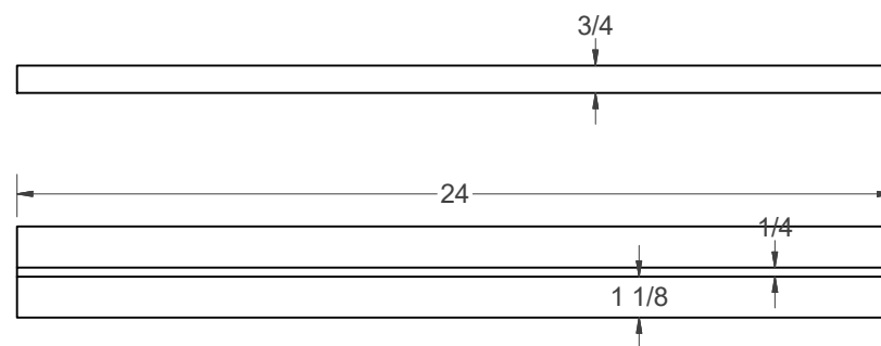
(E) - DRAWER SUPPORT
