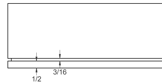
(N) - LARGE DRAWER SIDE (3 PCS)
