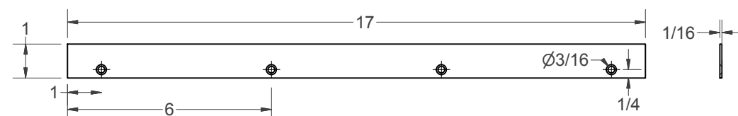
AKRO BIN HANGING BAR (5)
