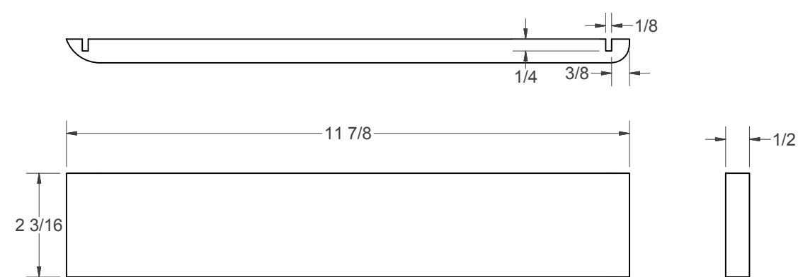
(I) - SMALL DRAWER END (4 PCS)
