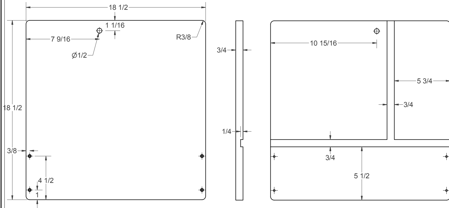
(A) - BOTTOM
