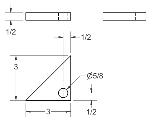
(L) - CORNER BLOCK (14 PCS)
