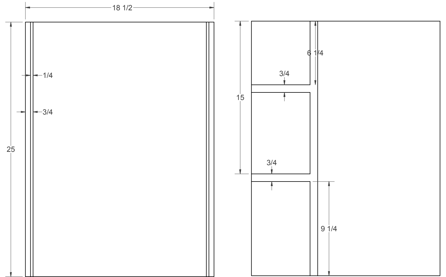
(B) - UPRIGHT
