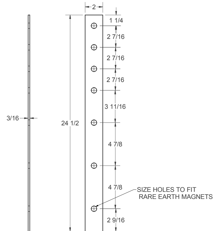
(O) - MAGNET STRIP
