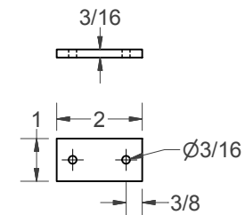
(P) - PLATE
