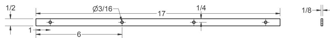
AKRO BIN RACK SPACER (5)
