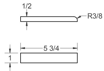
(G) - SHELF END (3 PCS)
