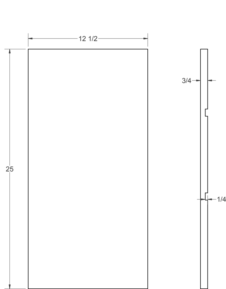
(C) - DIVIDER
