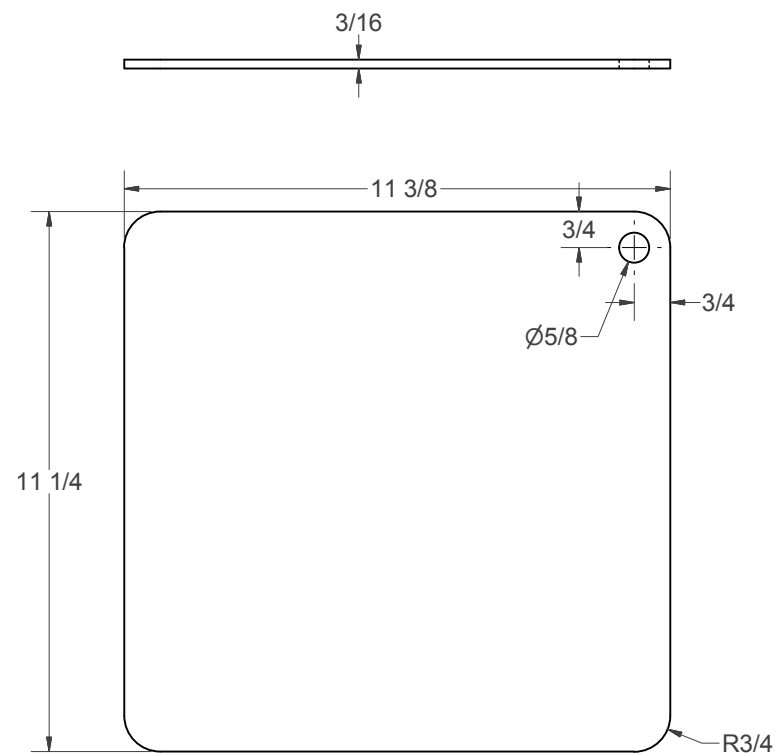
(K) - DRAWER BOTTOM (7 PCS)
