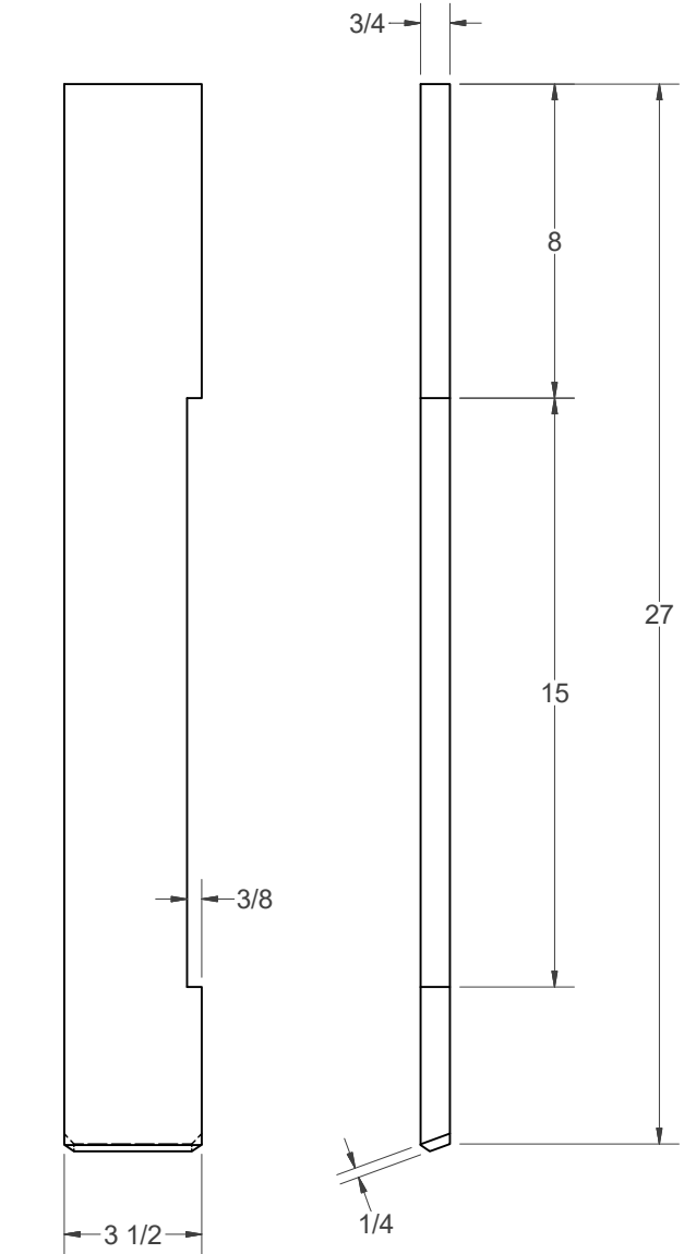
(A) - LEG OUTSIDE LAYER (4)
