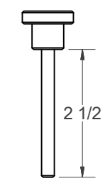
INDEX PIN
