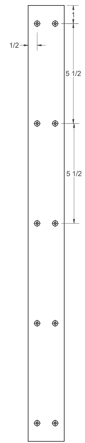
TRACK BED
