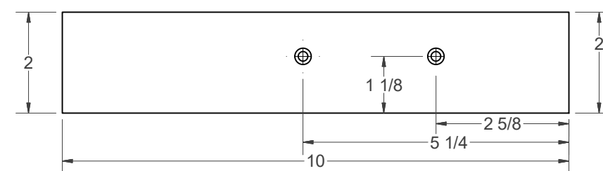
(G) - FENCE
