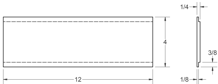
TRAY BOTTOM
