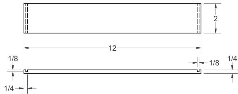
TRAY FRONT-BACK (2)
