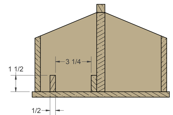
SECTION L-L
