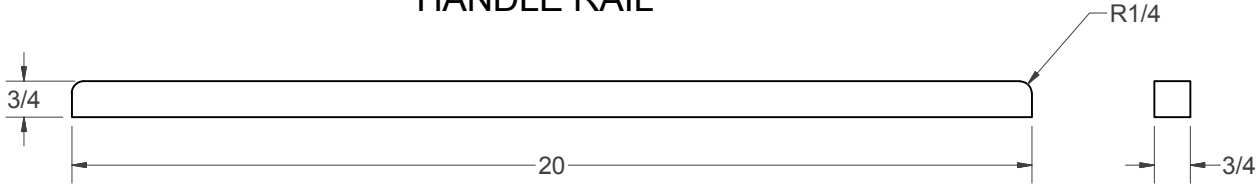
HANDLE RAIL
