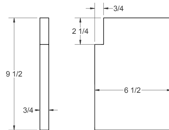
(O) - DIVIDERS (NEED 5)
