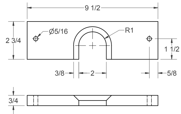
(P) - FENCE BASE
