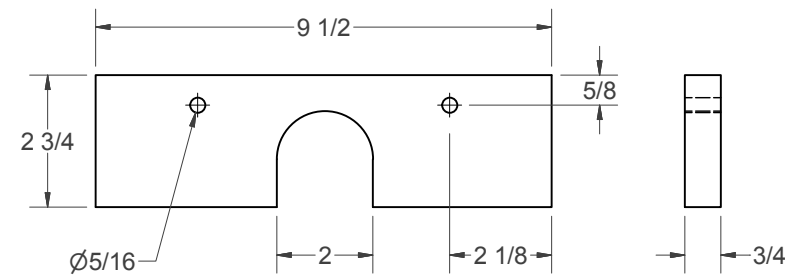
(Q) - FENCE BACK
