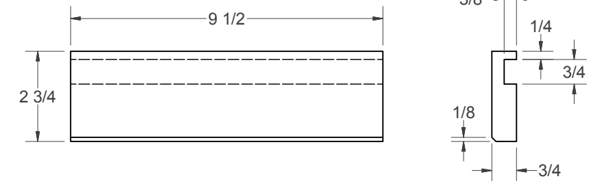
(R) - FENCE FACE (x2)
