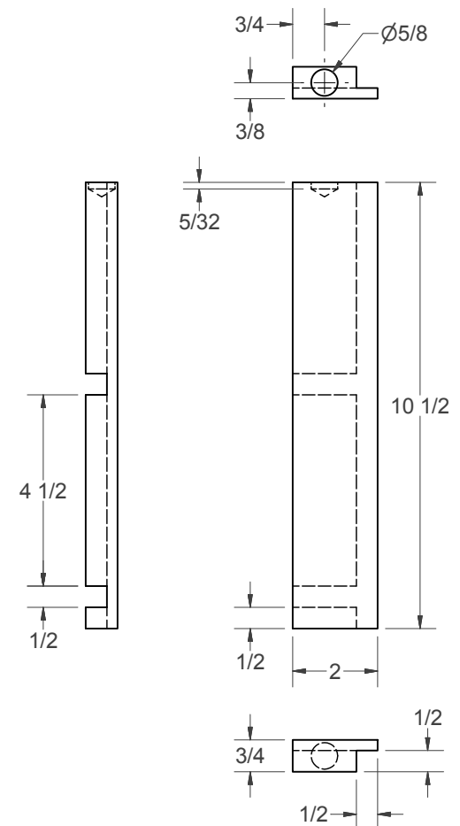
(F) - OUTER STILE
