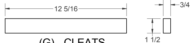
(G) - CLEATS (NEED 3)
