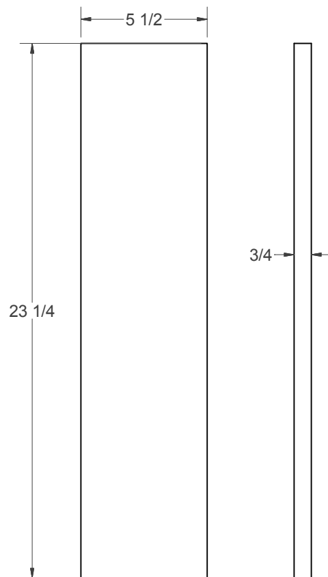
(C) - REAR DIVIDER (NEED 3)
