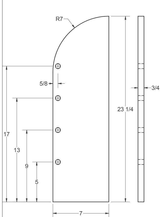
(A) - FRONT DIVIDER (NEED 2)
