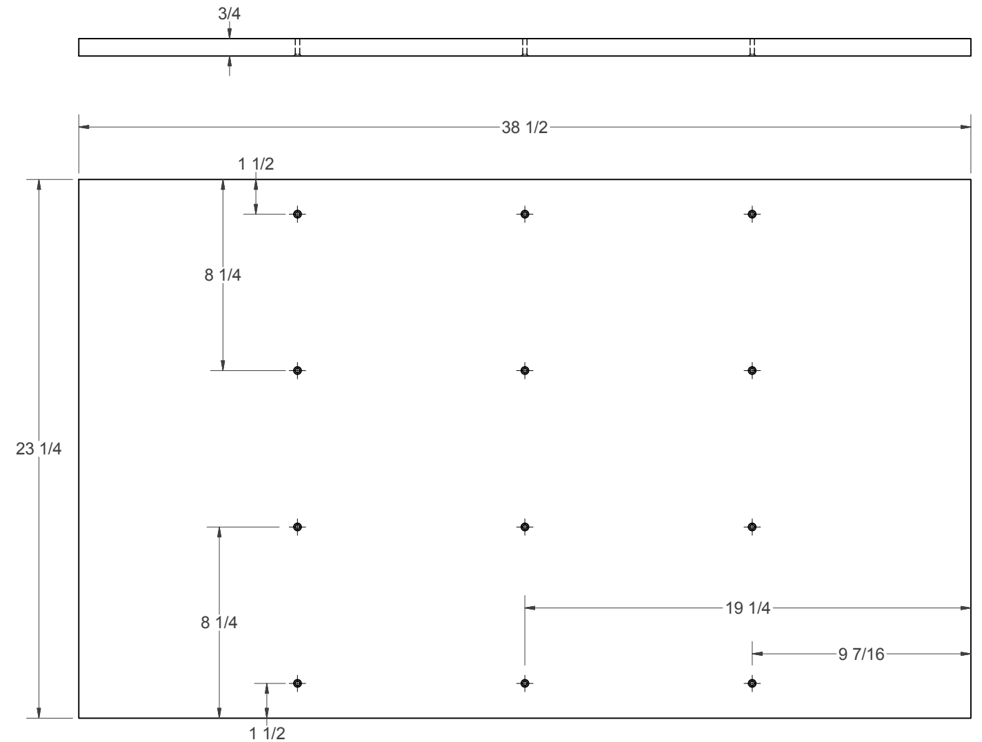
(B)- BIN BACK
