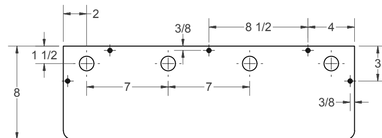
(Y) - RACK SHELF
