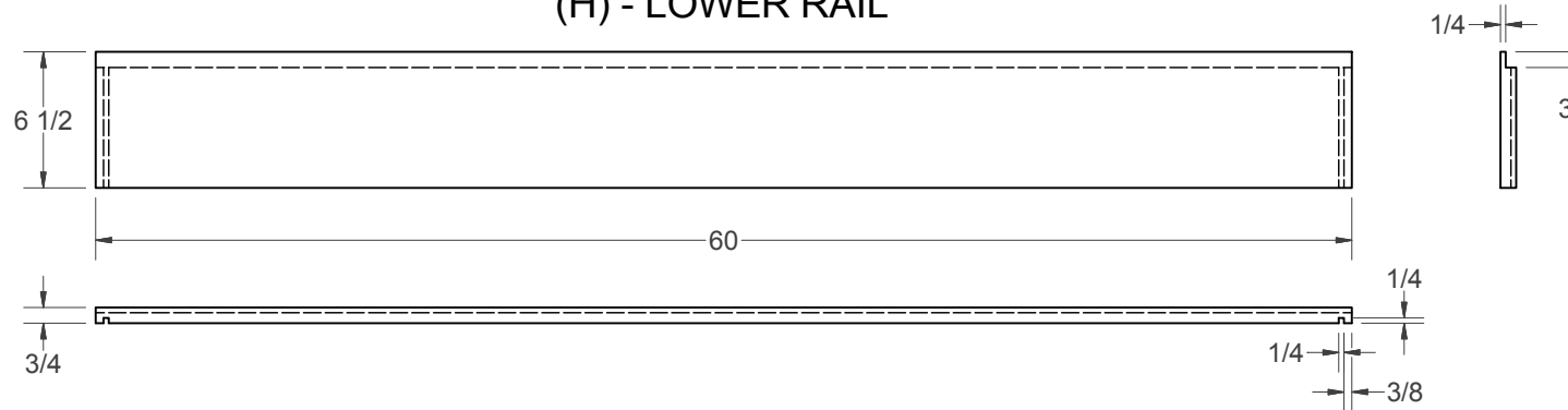
(H) - LOWER RAIL
