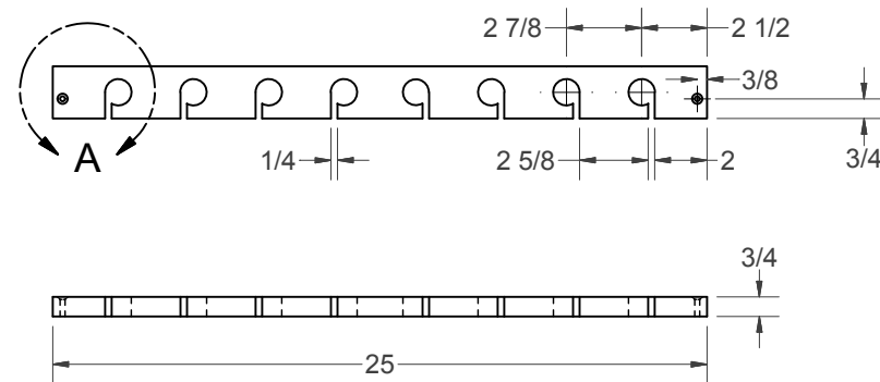
(BB) - CORD RAIL
