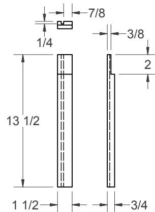
(K) - STILE (LEFT)
