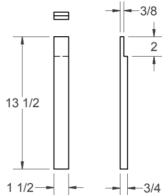
(K) - STILE (CENTER)
