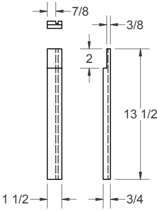
(K) - STILE (RIGHT)
