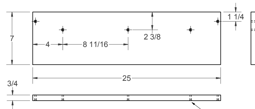
(Z) - RACK BACK
