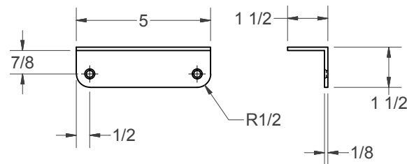
(V) - HANDLE BASE (6)
