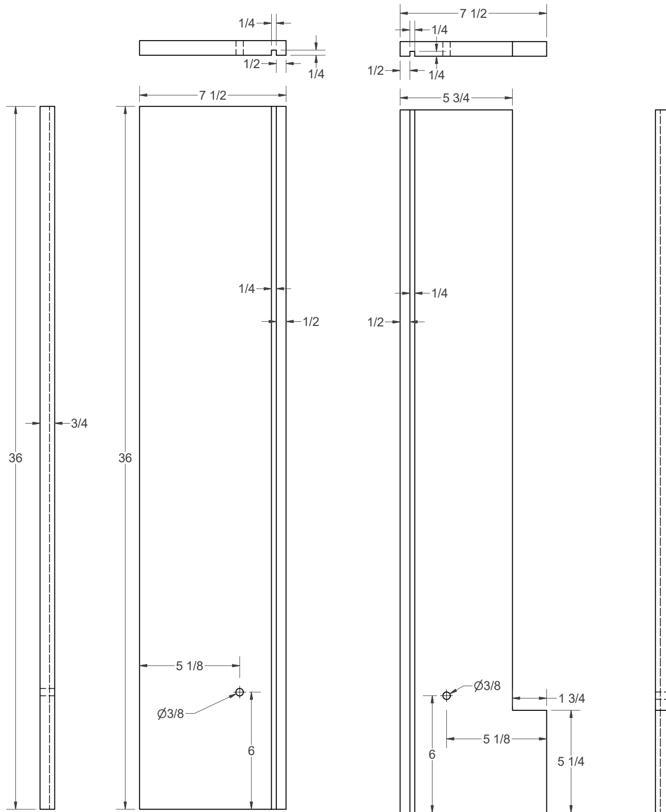
(A) - LEFT SIDE
