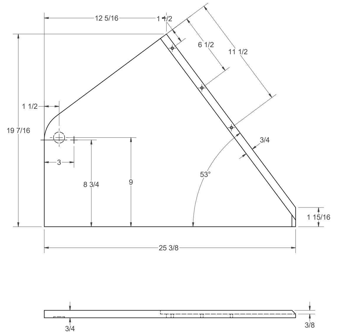
(P) - LEFT WING
