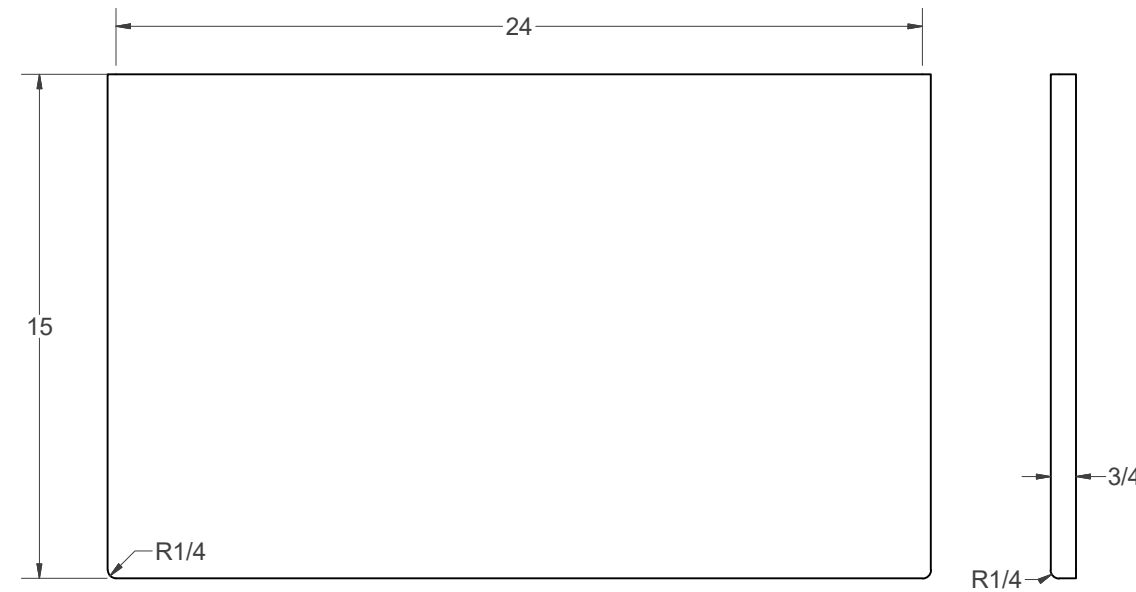
(M) - LOWER FILLER
