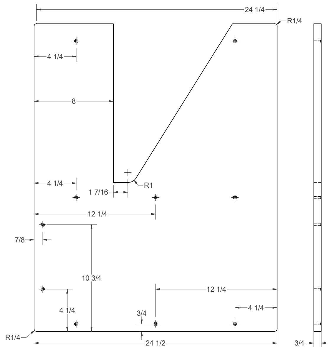
(E) - WING SIDE
