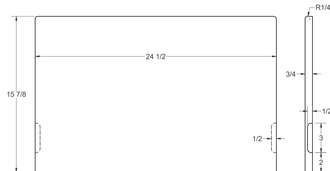
(L) - DROP LEAF
