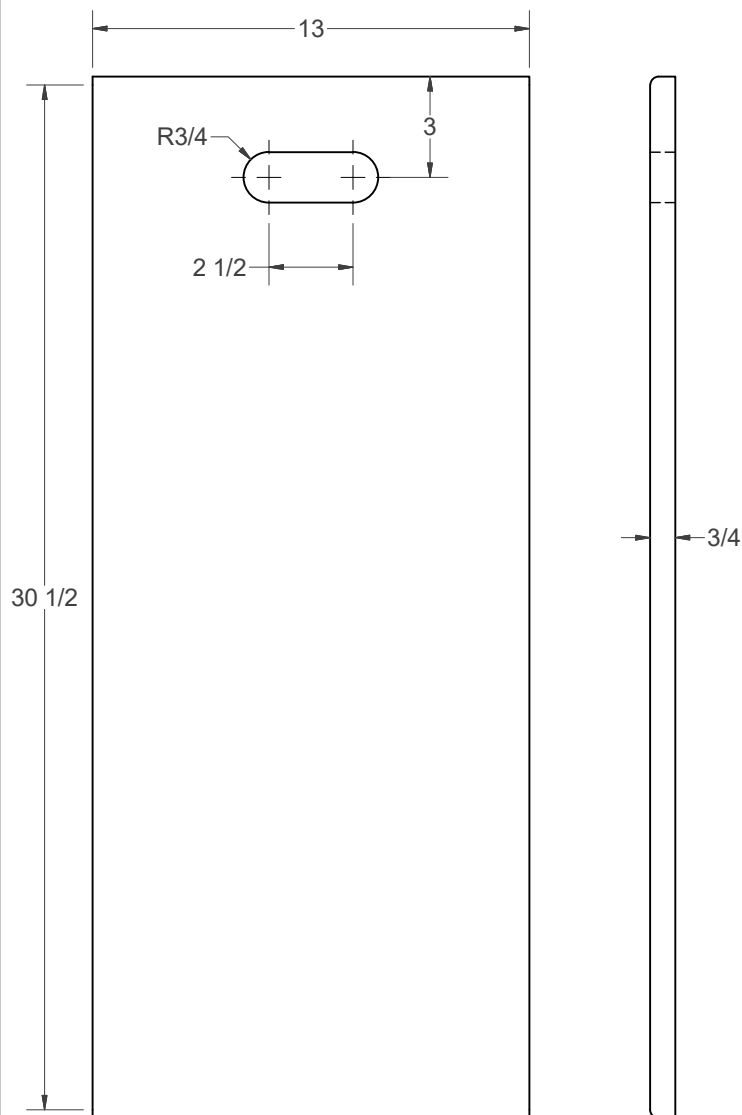
(H) - AUXILLARY TABLE
