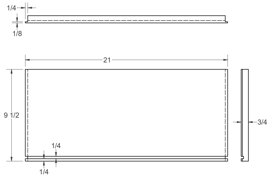
(O) - DRAWER BACK
