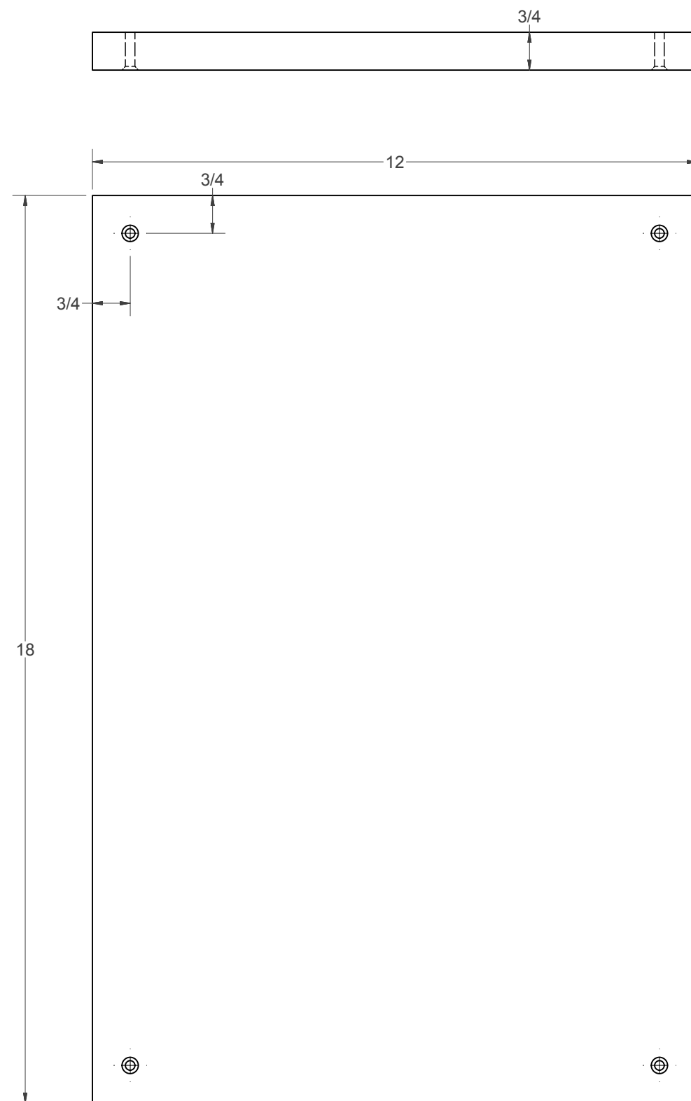
(B) - WORK PLATFORM
