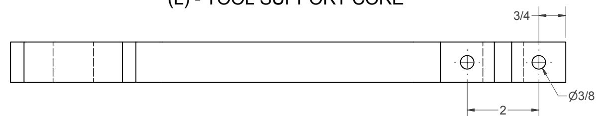
(L) - TOOL SUPPORT CORE
