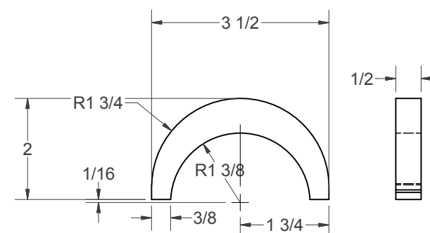
(N) - CLAMP BLOCKS (2 NEEDED)
