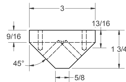
(F) - SHORT CARRIAGE BED (2 NEEDED)
