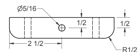
(H) - WHEEL RETAINERS (6 NEEDED)
