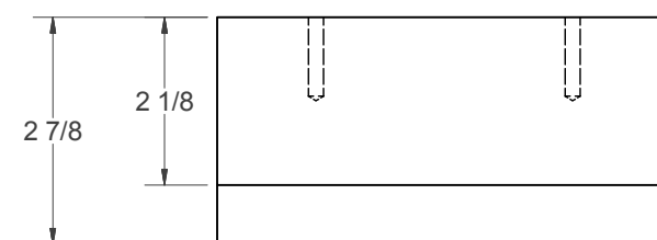
(G) - SHORT CARRIAGE SIDES (4 NEEDED)
