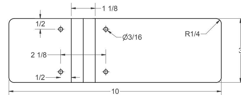
(F) - SHORT CARRIAGE BED (2 NEEDED)
